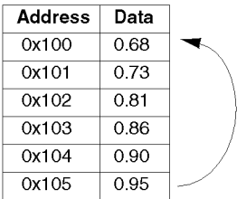
Figure 8-1. Example of Modulo Buffer
