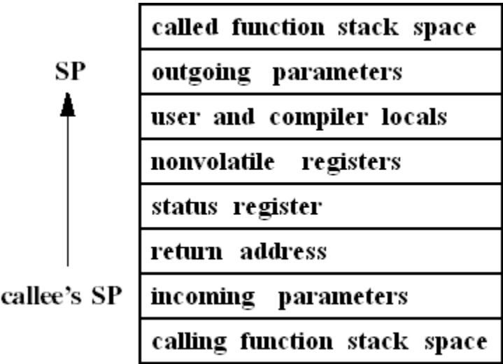
Figure 4-1. Stack Frame
