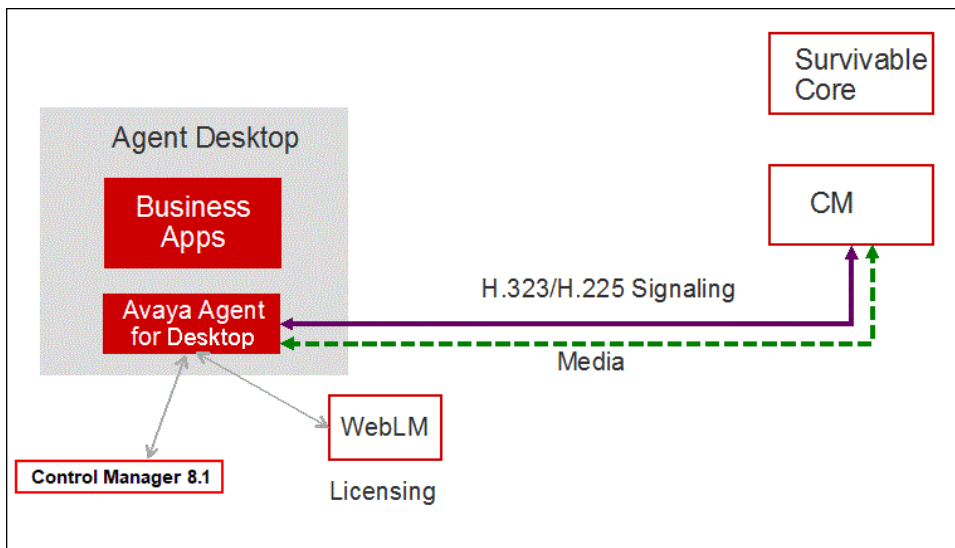
Figure 3: Standalone solution for H.323
