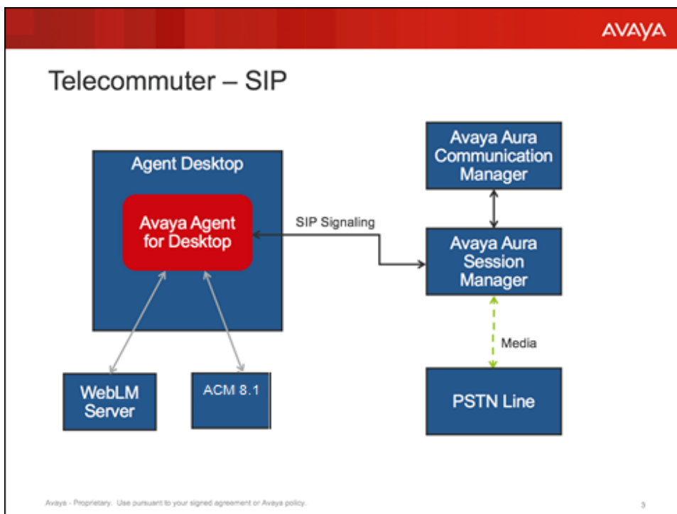
Figure 7: Telecommuter mode with SIP
