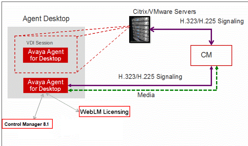
Figure 1: VDI solution with H.323
