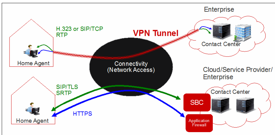
Figure 5: Remote agent solution for both VPN and SBC
