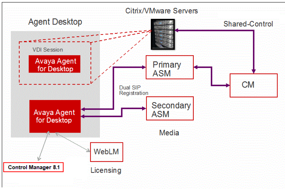
Figure 2: VDI solution with SIP
