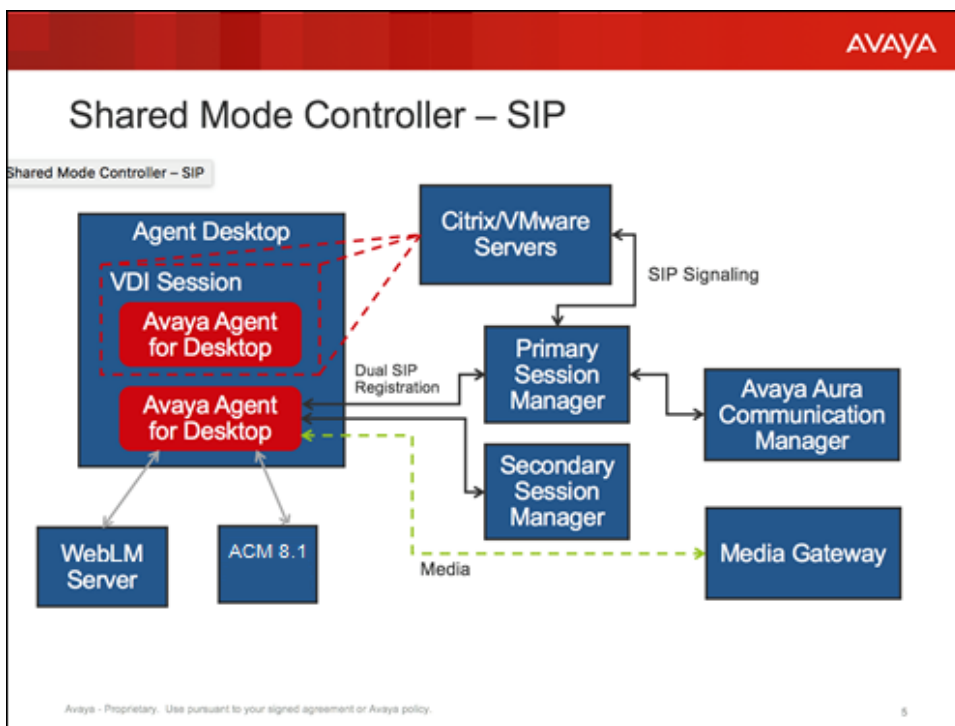
Figure 9: Shared Control as Controller with SIP
