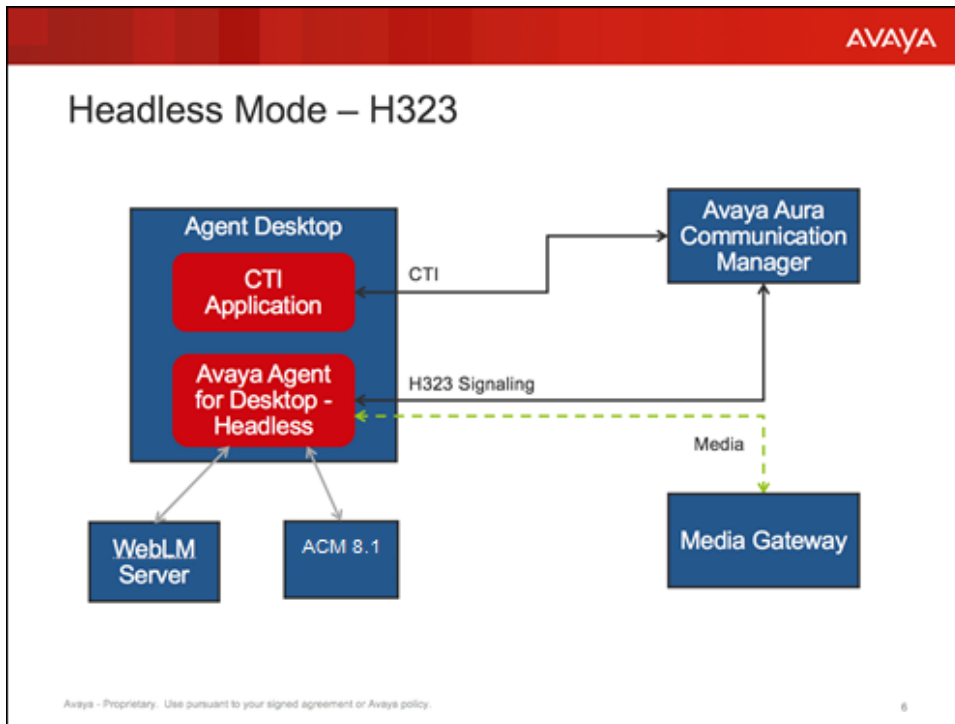
Figure 10: Headless Mode – H.323
