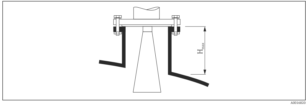
13 Nozzle height for horn antenna (FMR51)
