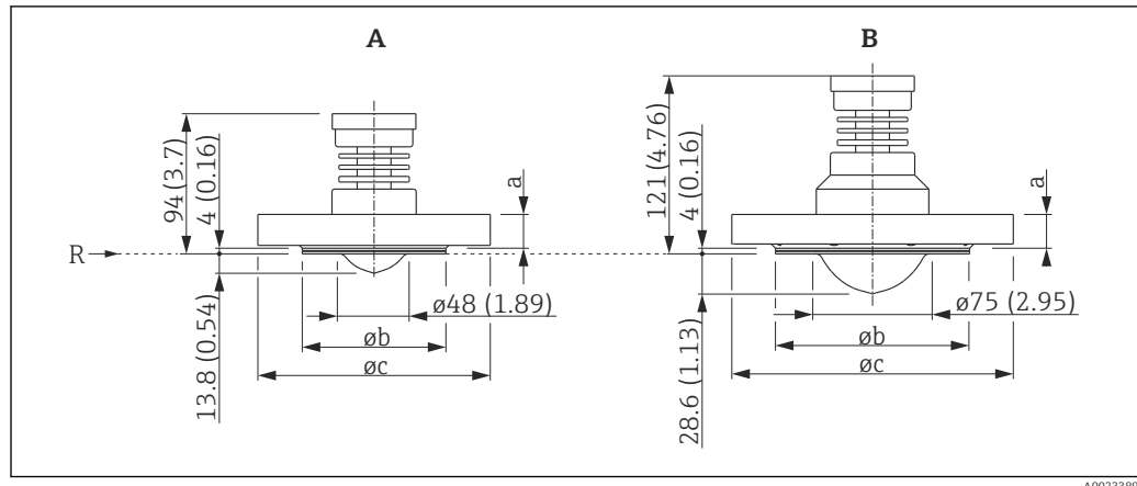
29 Dimensions FMR52 with flange; dimensions: mm (in)
