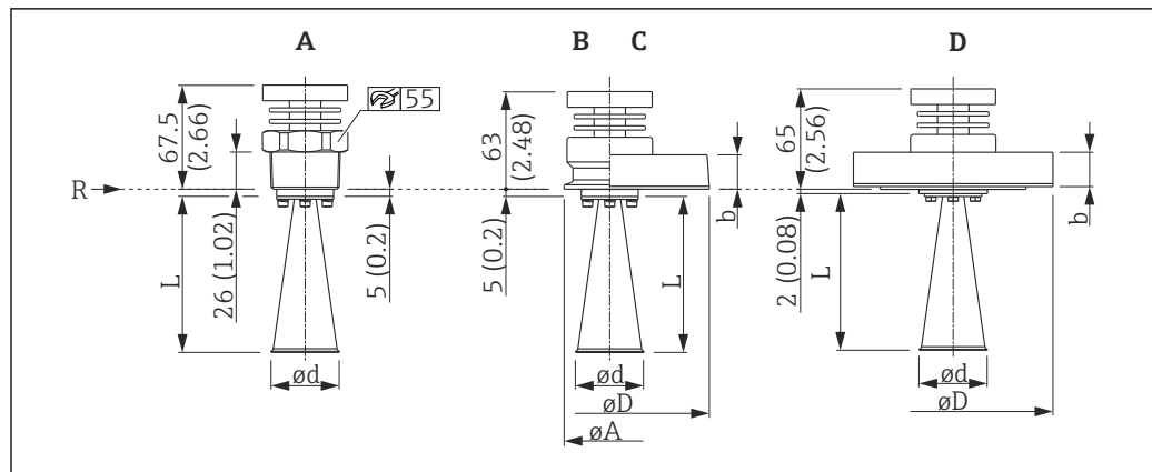
23 FMR51: Version T < 150\text{ °C} ( 302\text{ °F} ); without antenna extension; dimensions: mm (in)
