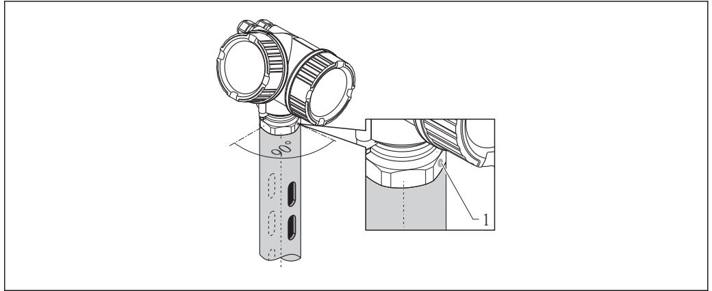
15 Installation in stilling well
