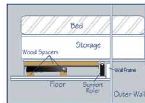
Fixed Frame - 5th wheel overhang
