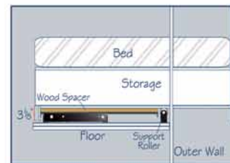
Fixed Frame - trailer application
