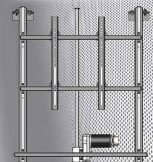
Lippert TV Lifts utilize a "power up/ power down" drive mechanism that operates smoothly without any "shake" or "shimmy."
