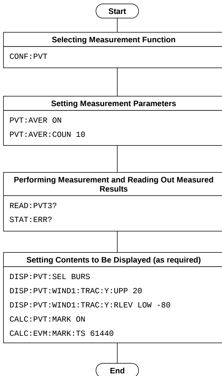
Figure 1.2.5-1 Flow of Common Settings for Modulation and Command Example
