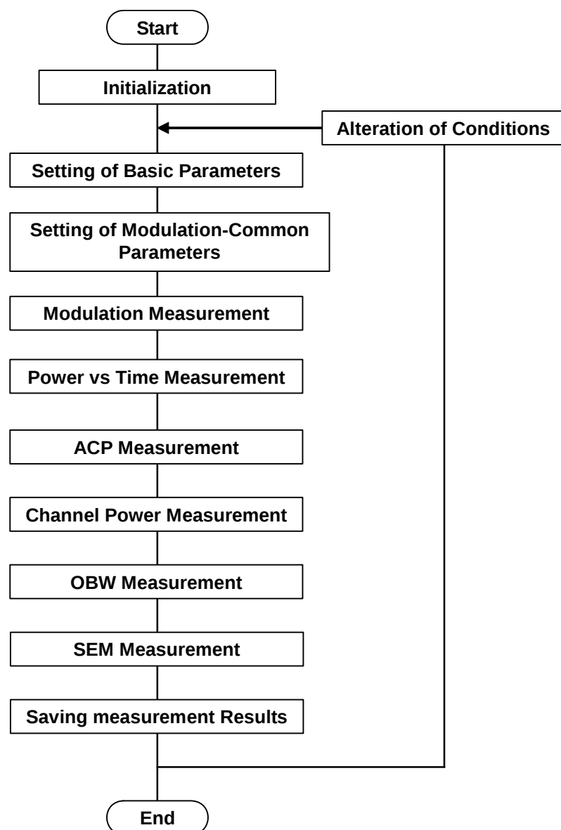
Figure 1.2-1 Flow of Basic Test
