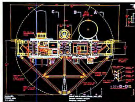
Materials Science Laboratory (MSL), attached to the support structure, shown on MicroStation PC
