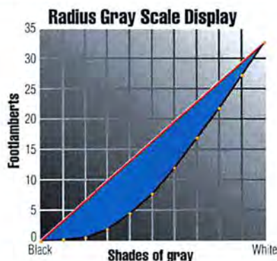
Radius Gray Scale Display gray shades
