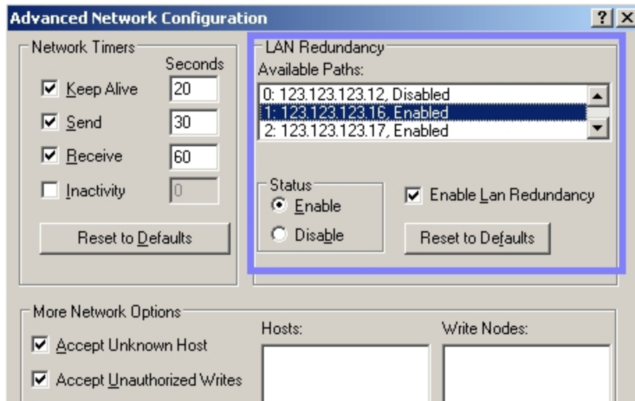
LAN Redundancy Portion of the Advanced Network Configuration Dialog Box in the SCU
