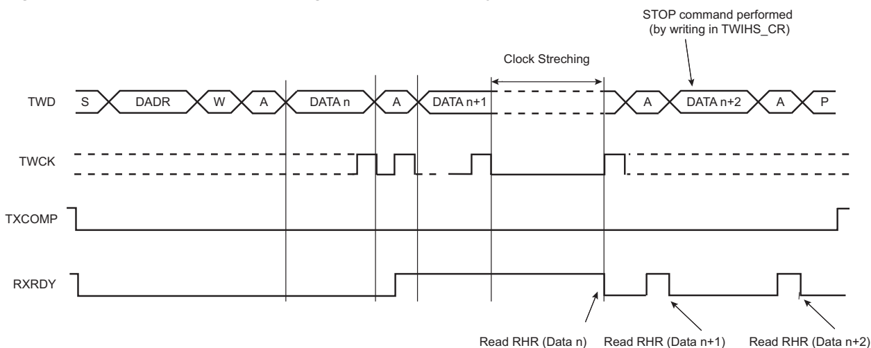
Figure 43-9. Host Read Clock Stretching with Multiple Data Bytes
