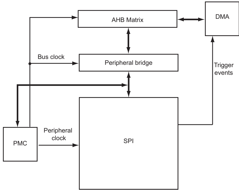
Figure 41-1. Block Diagram
