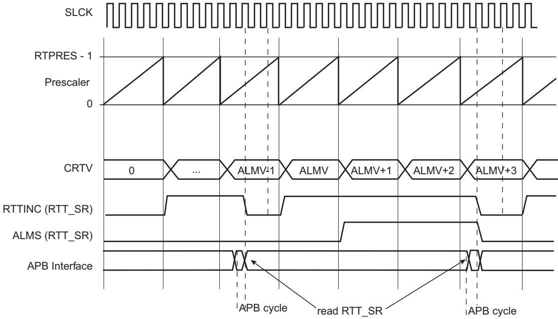
Figure 28-2. RTT Counting
