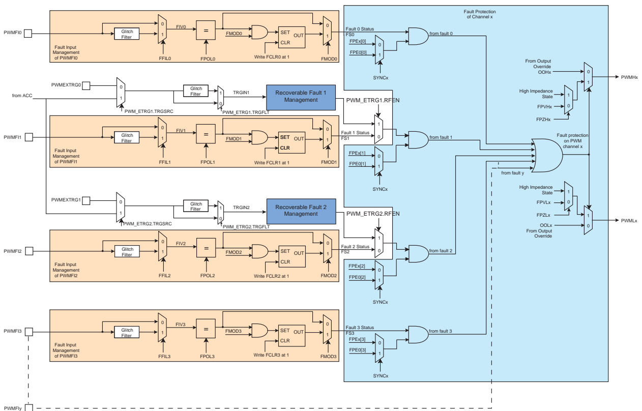
Figure 51-16. Fault Protection
