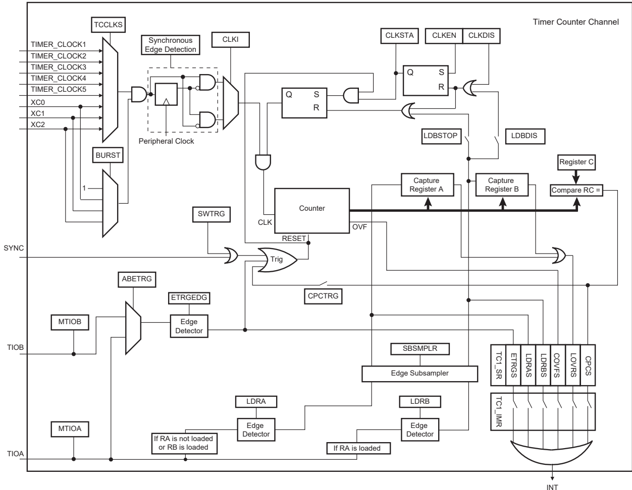
Figure 50-6. Capture Mode
