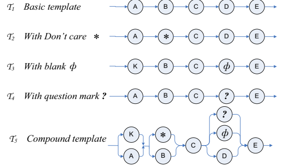
Figure 2: Illustration of templates
