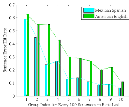
Figure 8: Auto-checking result on different speech database
