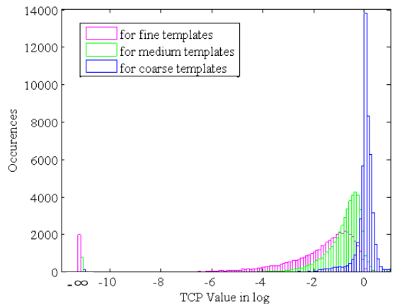
Figure 6: TCP value histogram for fine, medium, and coarse templates
