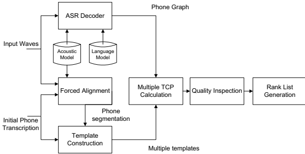
Figure 4: A flowchart of auto-checking procedure by TCP
