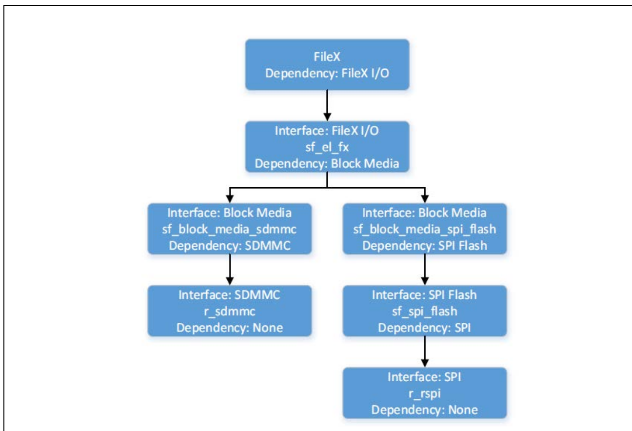
Figure 11 Connecting layers with the FileX interface
