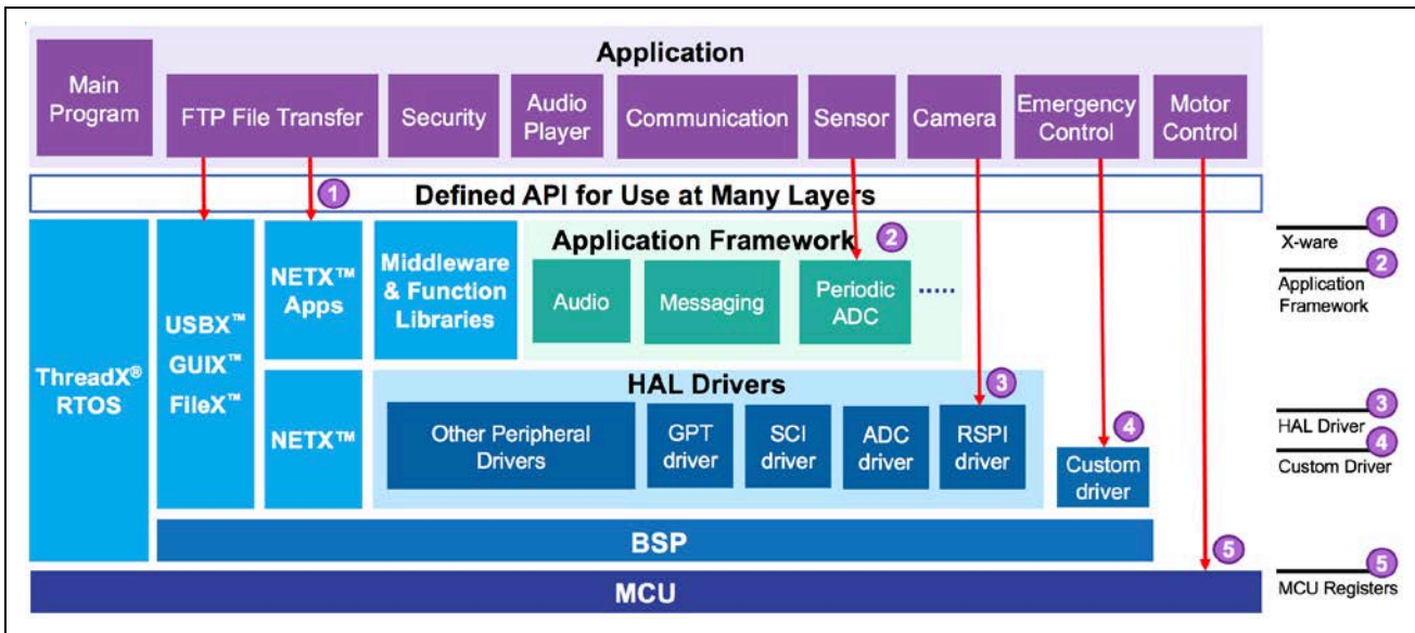
Figure 1 Software Architecture Overview
