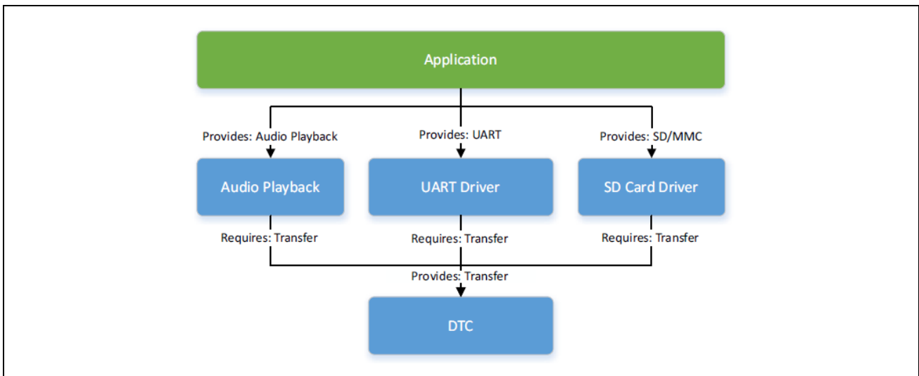
Figure 4 Example SSP stack
