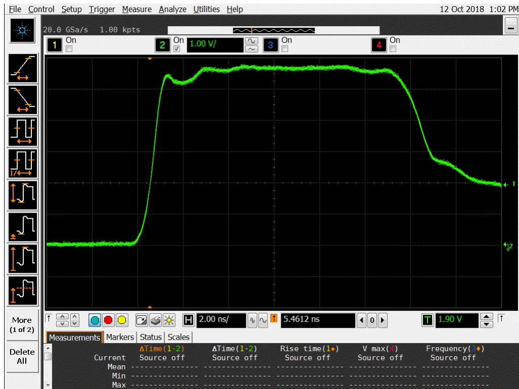
Figure 11a DUT 7403 Pre-Radiation Rising Edge
