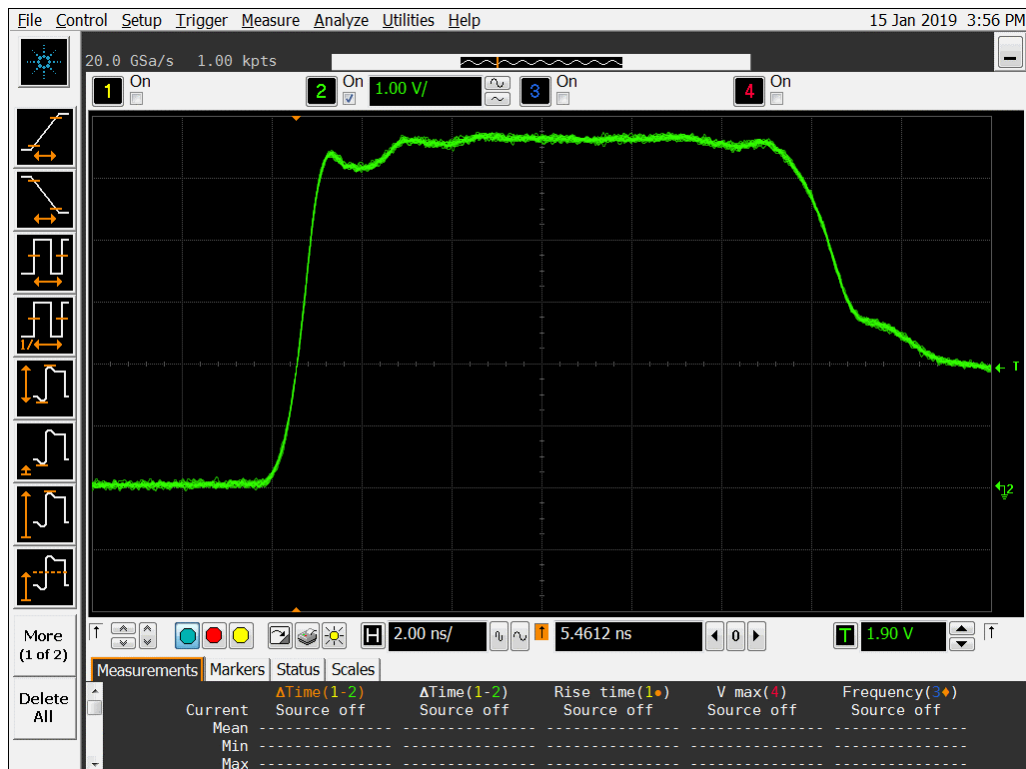
Figure 11b DUT 7403 Post-Annealing Rising edge
