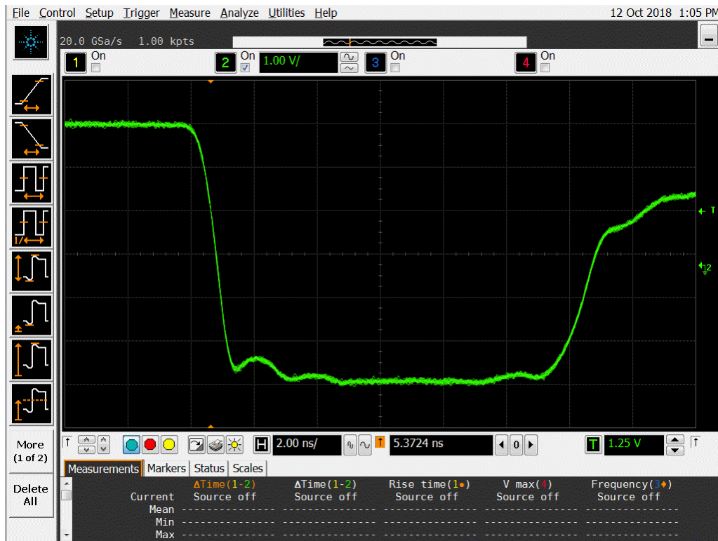
Figure 18a DUT 7407 Pre-Irradiation Falling Edge
