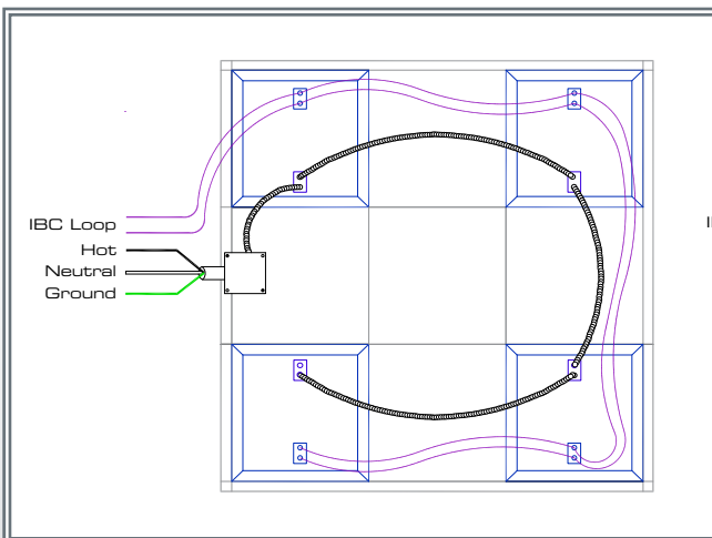
TRADITIONAL WIRING SYSTEMS
