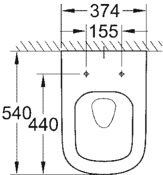
39 328 000 39 328 00H* WC suspendu Triple Vortex
