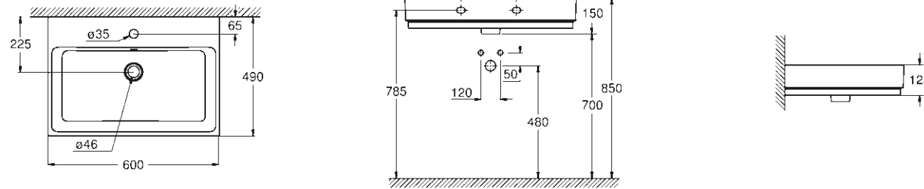
39 473 00H Lavabo suspendu 60 cm
