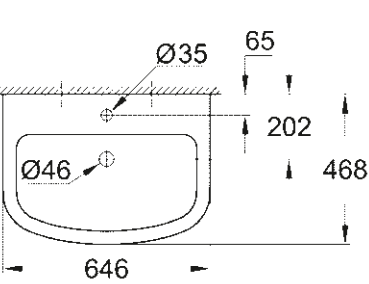
39 420 000 Lavabo suspendu 65 cm
