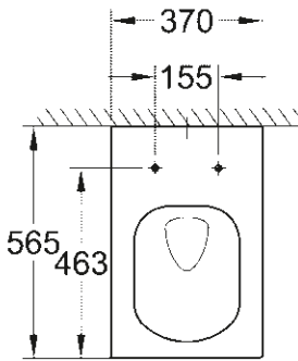
39 244 00H WC suspendu Triple Vortex
