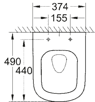
39 206 000 39 206 00H* WC suspendu compact Triple Vortex
