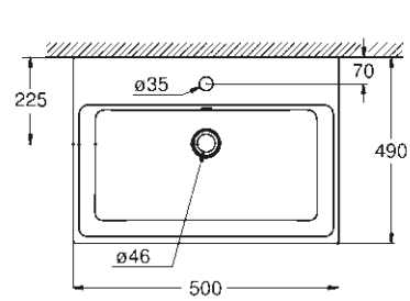
39 474 00H Lavabo suspendu 50 cm
