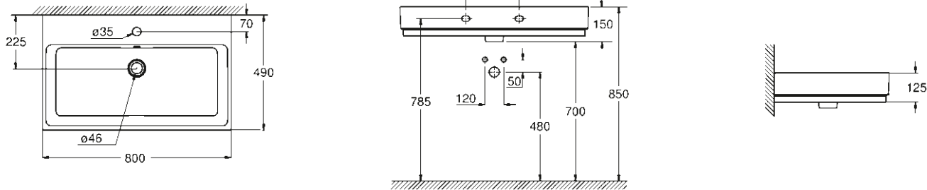
39 469 00H Lavabo suspendu 80 cm
