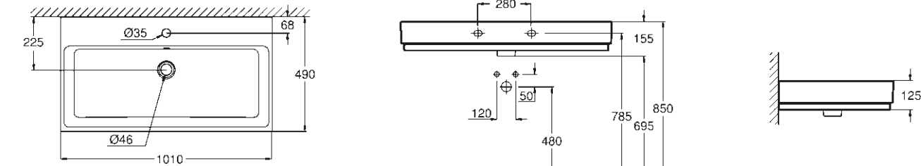
39 386 00H Lavabo suspendu 100 cm
