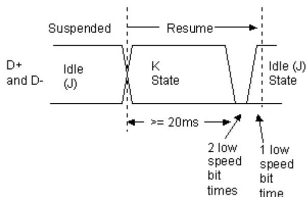
Figure 3. Resume timing
