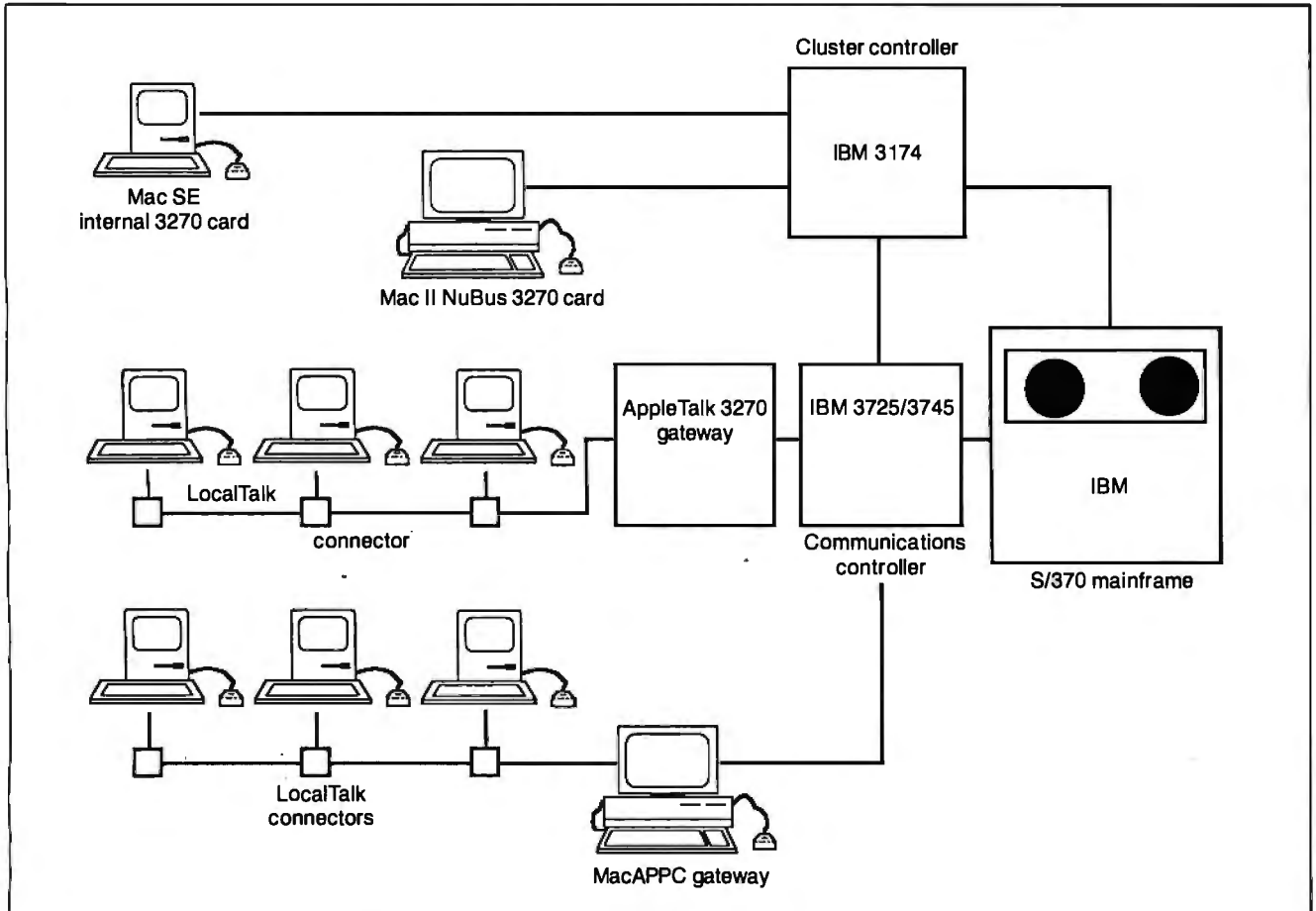
Figure 3: MacAPPC goes beyond 3270 terminal emulation and 3270 gateways to let the Mac act as an intelligent peer node on an IBM SNA network.
