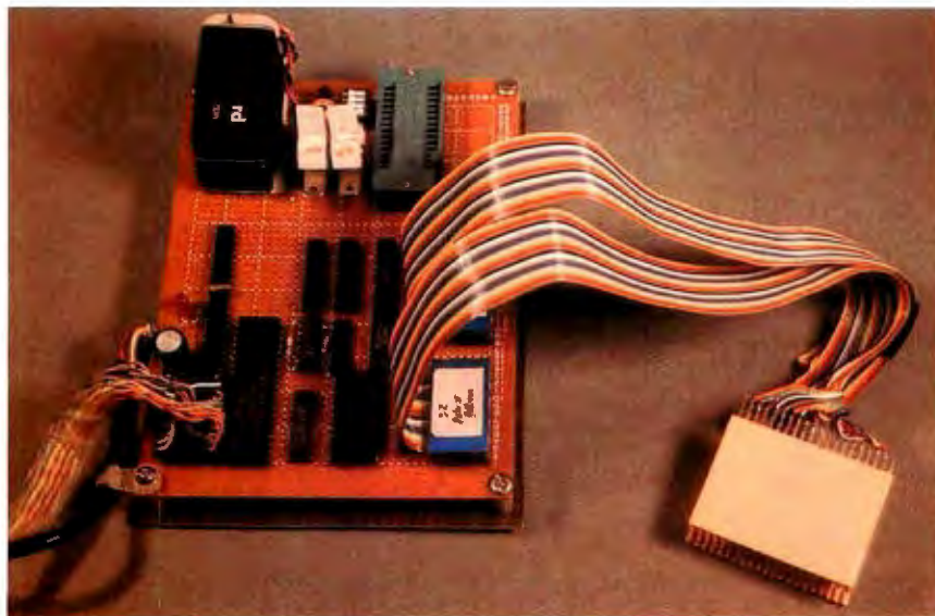
Photo 2: A prototype of the DDT-51 development system. Note the DIP clip at the end of the cable for attaching onto the target system's processor.
