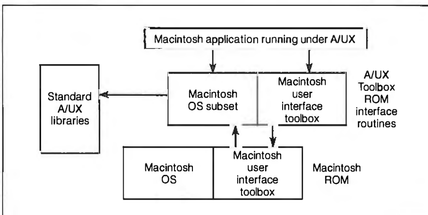
Figure 1: The strategy A/UX uses to communicate between an A/UX C program and the Mac ROM. If the C program makes a call to the Mac operating system, the Toolbox routes the call to an equivalent A/UX kernel function; if the program calls a Mac user interface routine, the Toolkit does an A-line trap to the Mac ROM.
