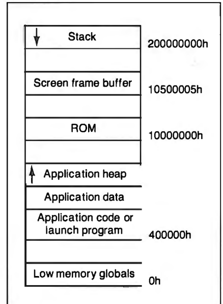
Figure 2: Except for the low-memory globals, none of the addresses that A/UX uses are the same as the ones used by the native Mac operating system. This doesn't matter, since everything is referenced through pointers in memory.
