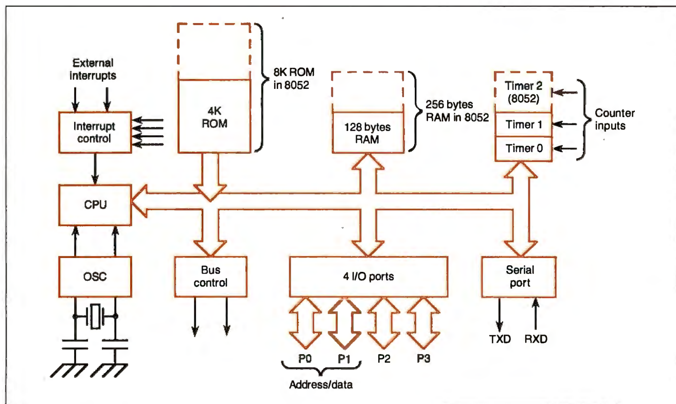
Figure 1: Inside the 8051.
