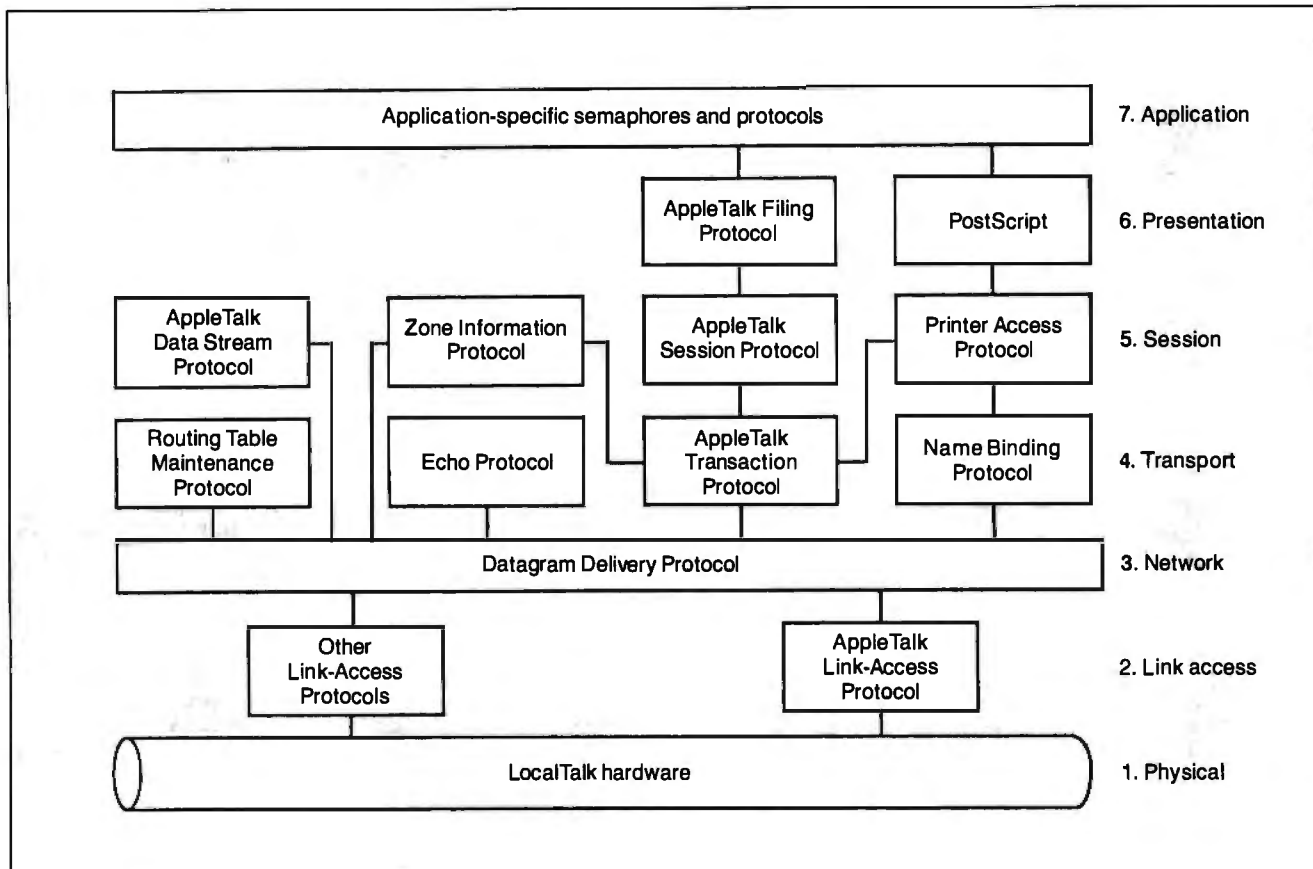
Figure 1: AppleTalk's seven-layer architecture is similar to that of the OSI reference model. The protocols, however, are proprietary.
