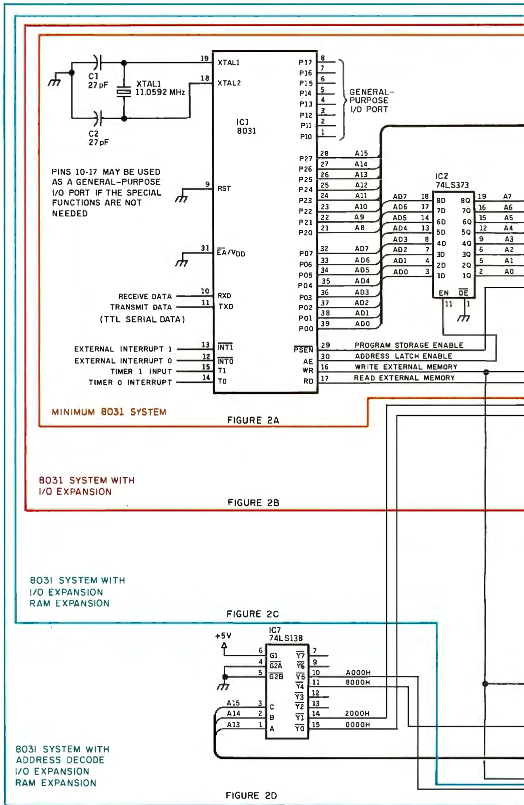
Figure 2: Growing an 8031 system. (a) A minimum configuration, (b) minimum system with I/O expansion, (c) system with I/O and RAM expansion, and (d) system with address decode logic and even more RAM and I/O.
