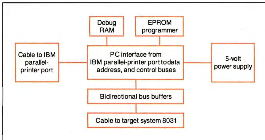
Figure 3: A block diagram of the DDT-51 8031/8051 development system.
