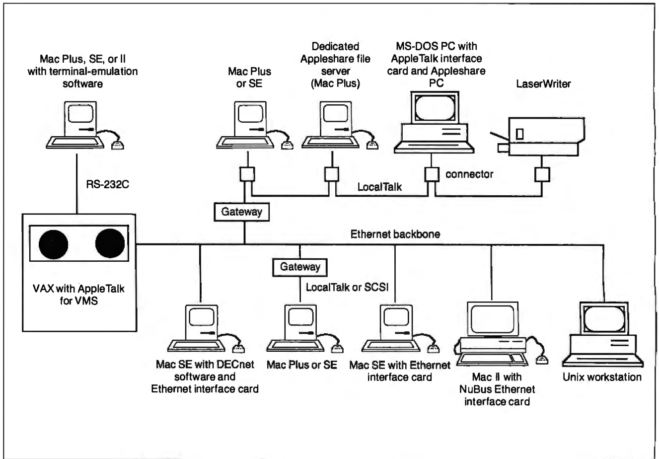
Figure 2: Macs connected to DECnet's Ethernet backbone can function as DECnet nodes, or the VAX can act as an AppleTalk file server.
