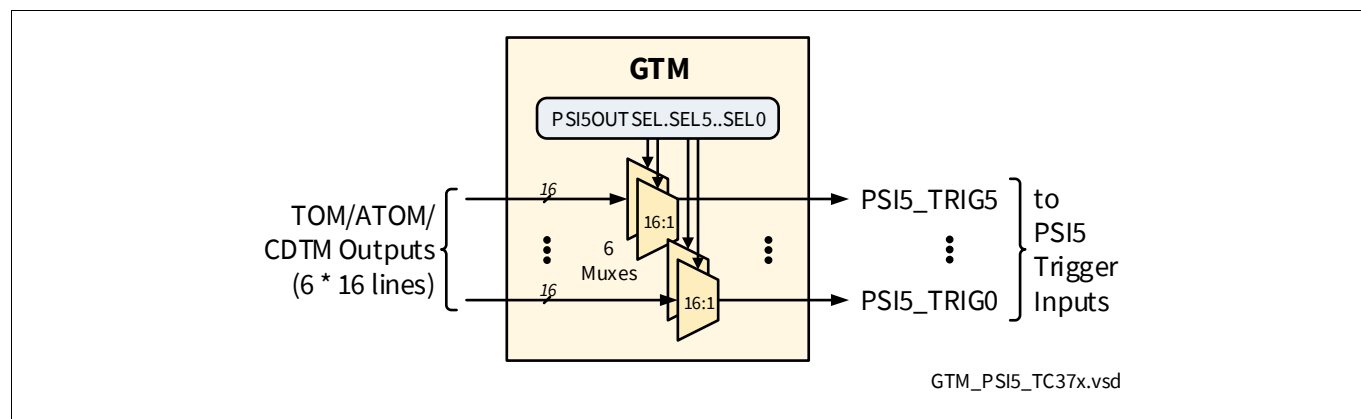
Figure 24 GTM to PSI5 Connections Overview
