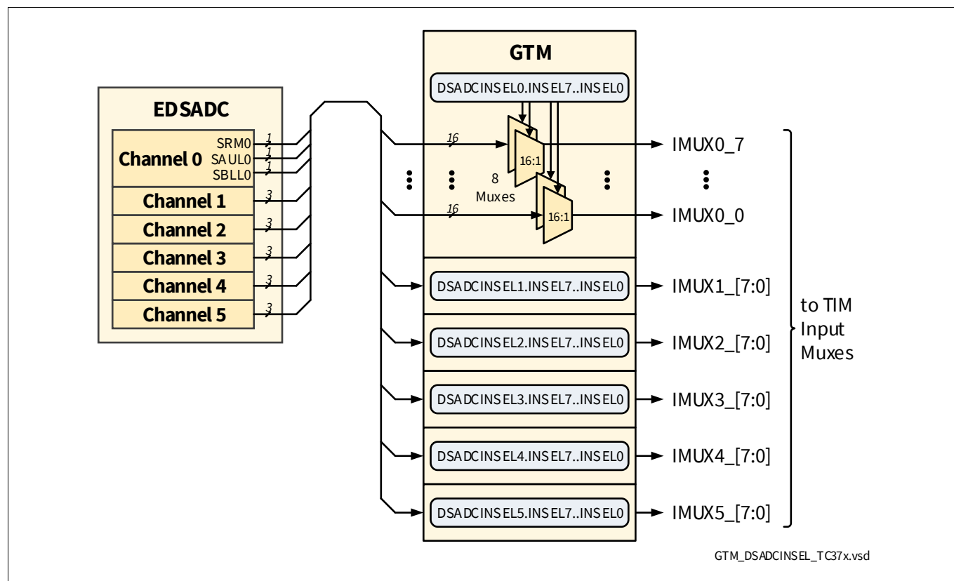
Figure 16 EDSADC to GTM Connections Overview
