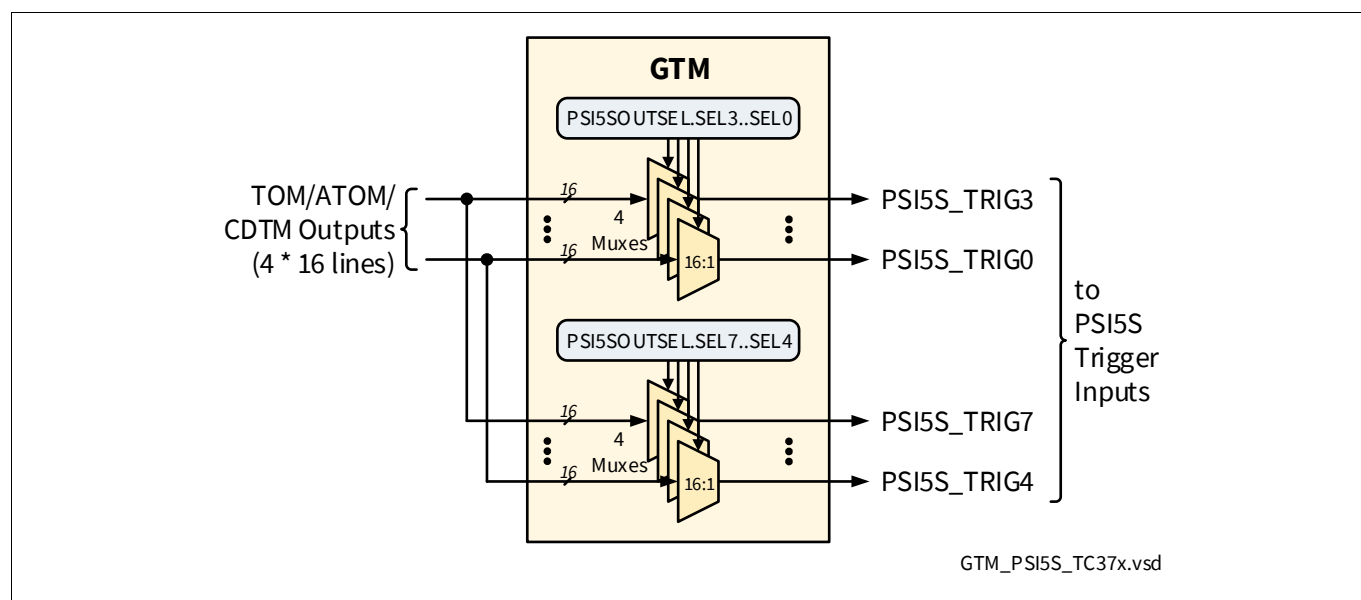
Figure 25 GTM to PSI5S Connections Overview
