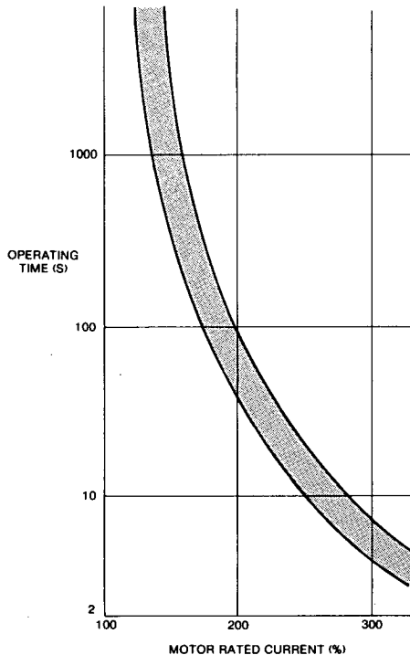
Fig. 6.12 Overload Characteristics
