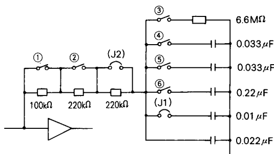
Fig. 6.15 Speed Amplifier PI Constant (SW3-① to ⑥)
