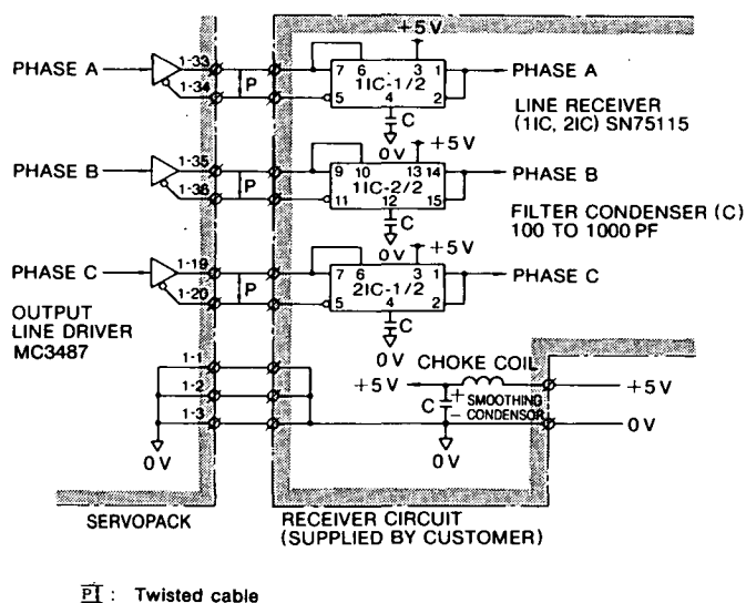
Fig. 6.8 Output Circuit and Receiver Circuit
