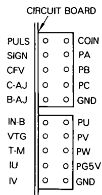
Fig. 6.18 Check Terminal Arrangement
