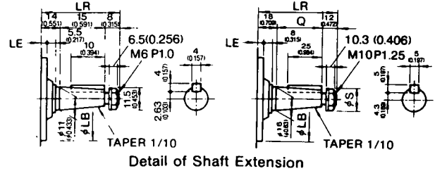
Detail of Shaft Extension
