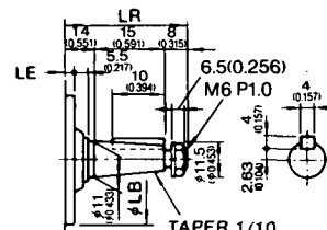
Detail of Shaft Extension
