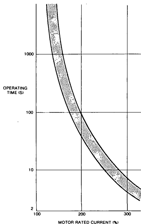
Fig. 4.1 Allowable Conduction Current of Servopack.
