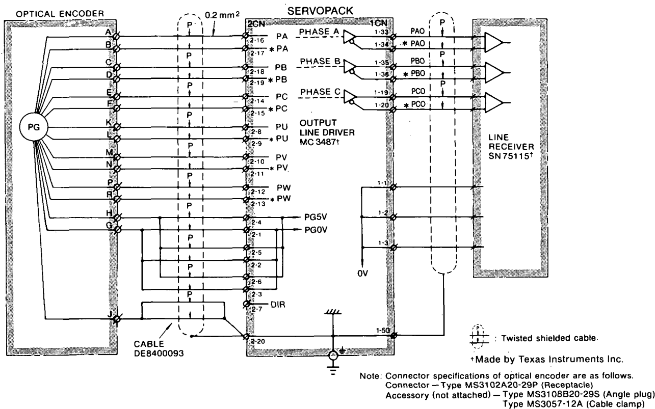
Fig. 5.5 Caulking Type Connector 2CN Connection and 1CN Output Processing (when using Connection Cable DE8400093)
