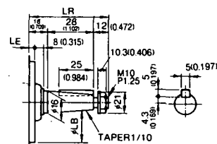
Detail of Shaft Extension
