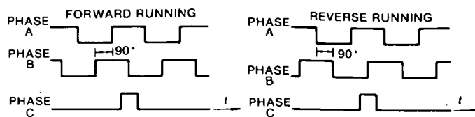
Fig. 6.9 Output Phase
