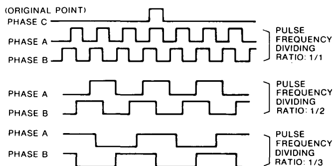
Fig. 6.10 Output Waveform of Optical Encoder
