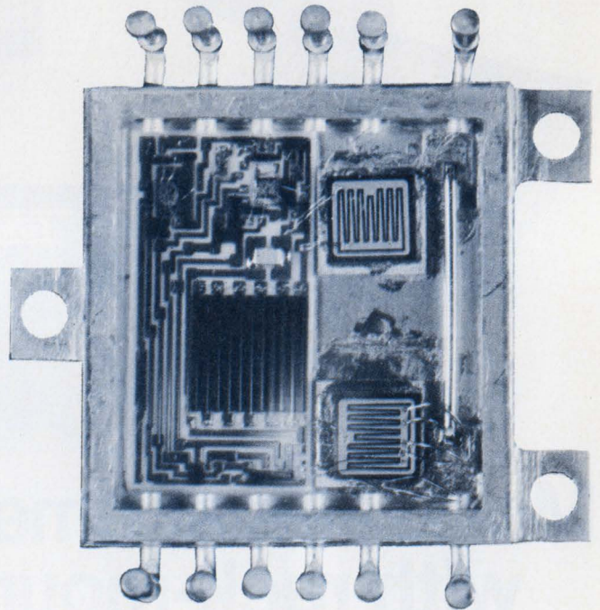
1. A complete 100-W series regulator fits into the "squared off" volume of one of the two TO-63 power-transistor packages required in the equivalent discrete design. (Several external resistors are shown in Fig. 3b.) The large dark area is a 2-W large-area film resistor, required in this positive regulator.
