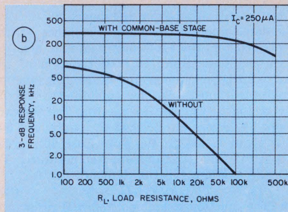
8. Improved frequency response of a phototransistor is obtained with a common-base load-impedance transforming network (a) in either the collector or emitter circuit. The degree of the improvement is shown in "b".
