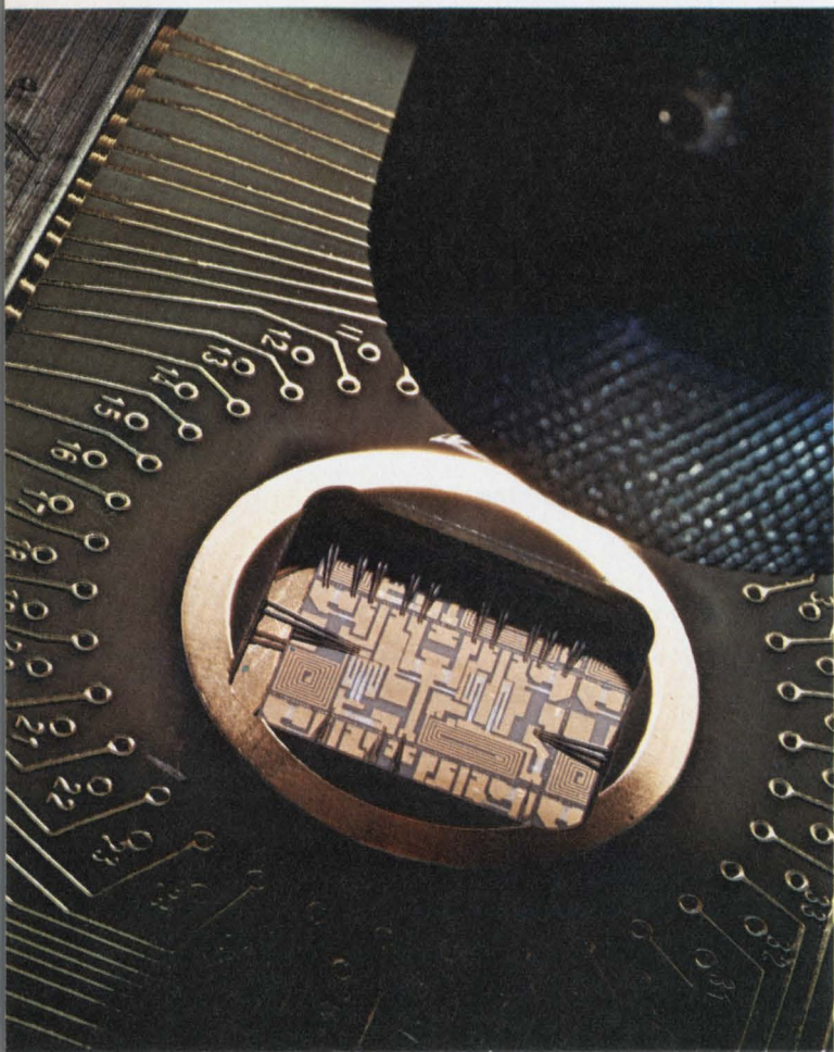
At Motorola Semiconductor, a two-stage complementary symmetry line extender is trimmed on a laser system. The thin-film hybrid includes inductors (square loops).
