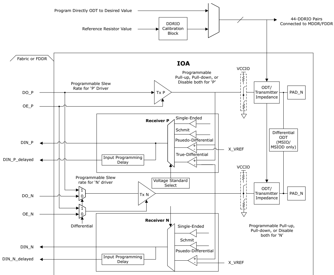
Figure 2 • IOA Architecture
