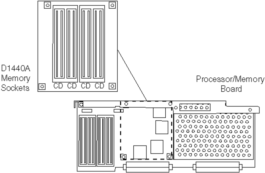
D1440A Vectra QS Main Memory Extension Board
