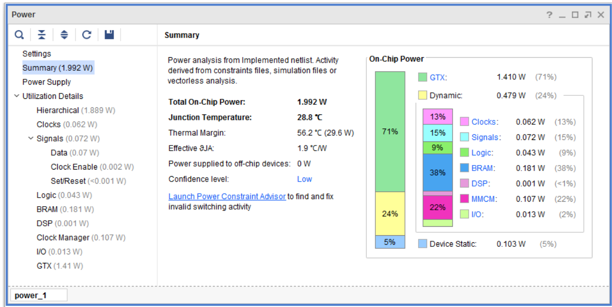
Figure 167: Power Report
