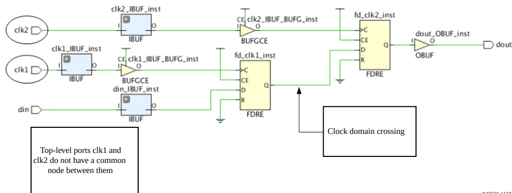
Figure 229: No Common Node Between Related Clocks
