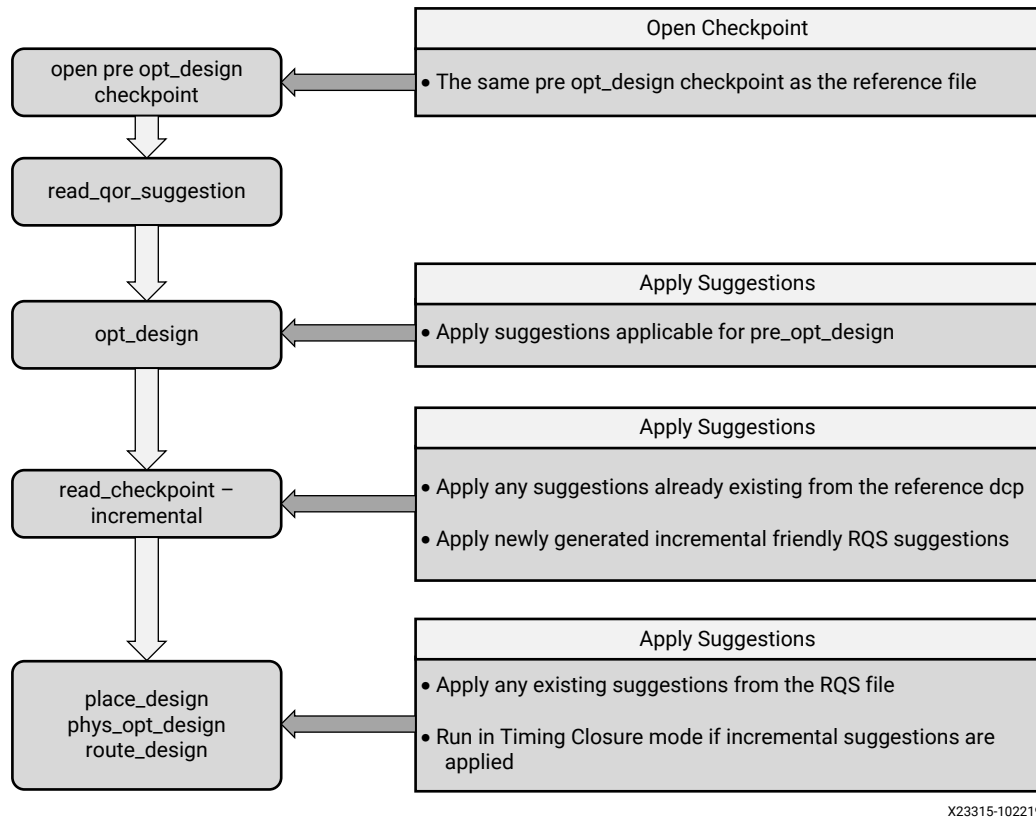
Figure 122: Incremental Flow
