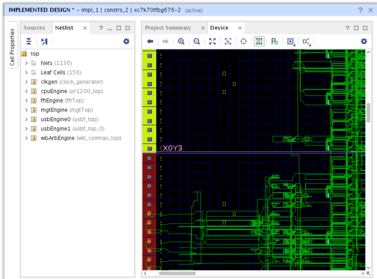
Figure 92: Abstract View
