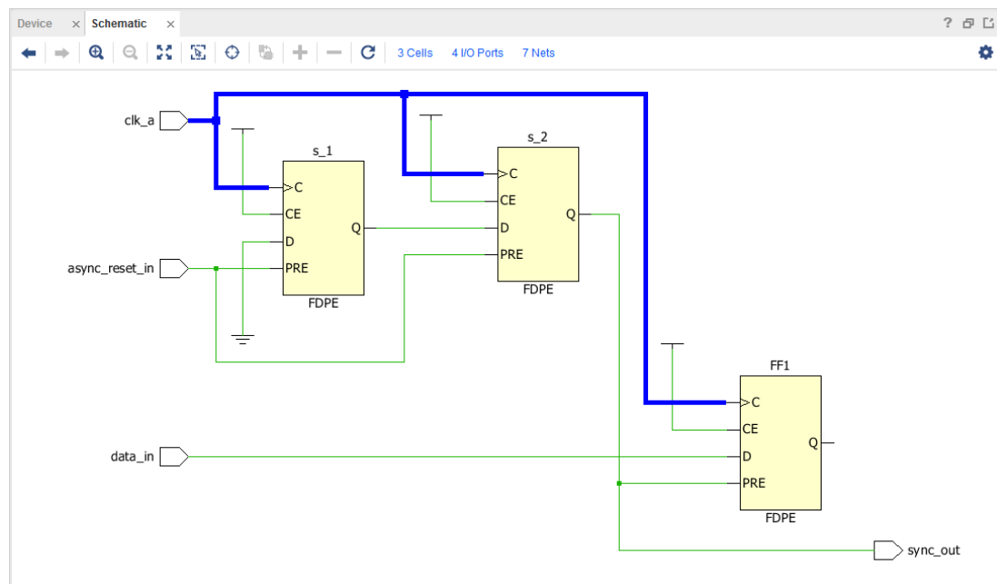
Figure 69: PRESET-Based Asynchronous Reset Synchronizer
