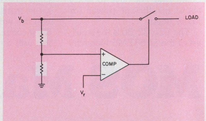
1. Popular load-cutout circuits compare the battery voltage ( V_b ) to a fixed reference voltage ( V_r ). The load is disconnected when the battery voltage gets too low.
