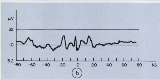
3. Response changes severely in an MC 4044 detector (a) within its zero-phase-error region and over a 150-ns range of delays between the inputs. With 90^\circ offset inputs, response (b) shows interaction.
