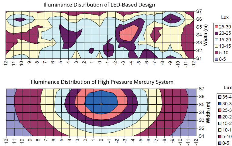
Figure 4. Light distribution of LEDs versus mercury vapor.
