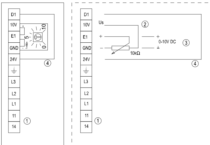
Internal potentiometer
