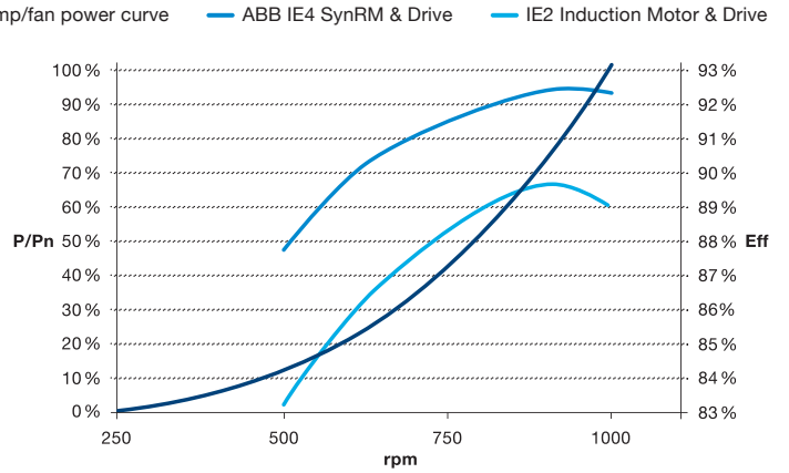
37 kW, 1000 rpm, drive system in pump/fan duty
