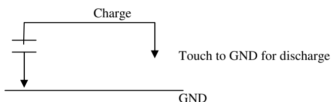
Figure 6.0-3: Basic Charge Device Model equivalent circuit
