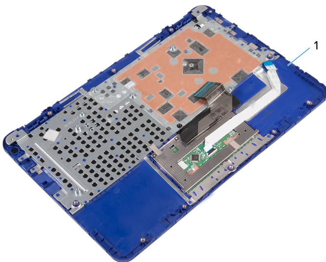
Figure 31. Palm-rest and keyboard assembly
