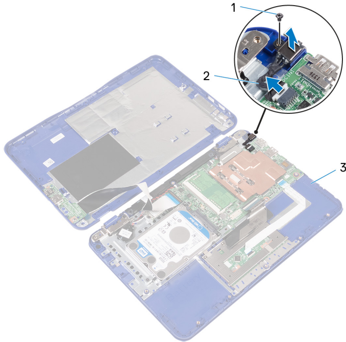
Figure 19. Removing the power-adaptor port
