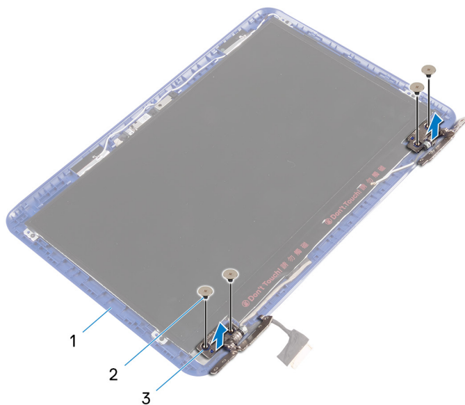
Figure 34. Removing the hinges
