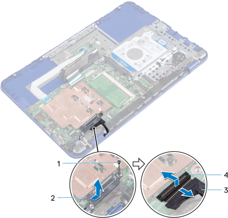
Figure 24. Removing the display cable
