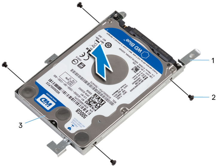
Figure 18. Removing the hard drive
