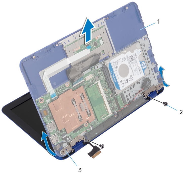
Figure 26. Removing the display
