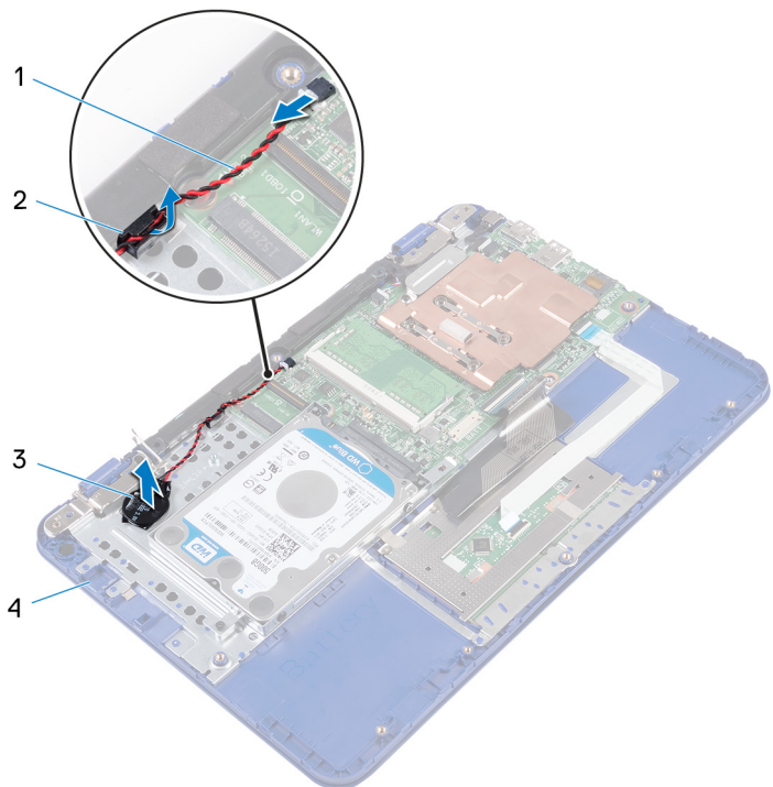
Figure 22. Removing coin-cell battery
