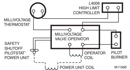
Fig. 27. Typical Powerpile® System wiring diagram.
