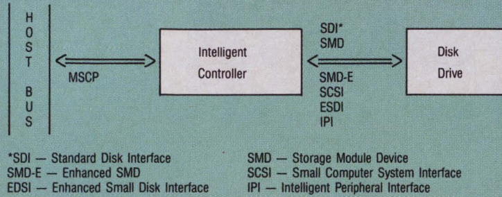
Disk storage system architecture.
