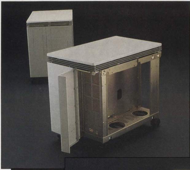
The expansion cabinet takes a BA 23, which resolves any DEC-related service issues.
