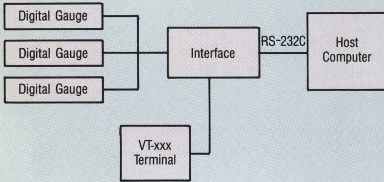
Concept for automatic quality data collection.
