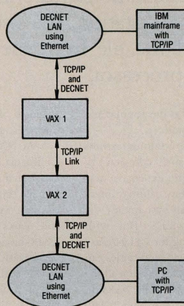
An organization running two DECNETs in separate cities, each with a VAX supporting its own Ethernet LAN, with several local workstations.
