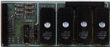
A plug-in "personality module" tells the 600 Series whether to emulate a DEC, Wyse, Televideo or you-name-it.
