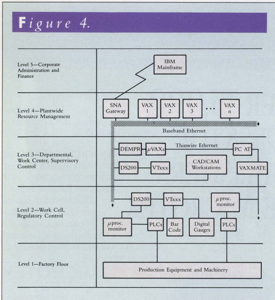
Simplified diagram of a CIM topology.
