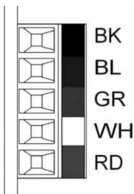
Fig 1.3 – DeviceNet Connector
