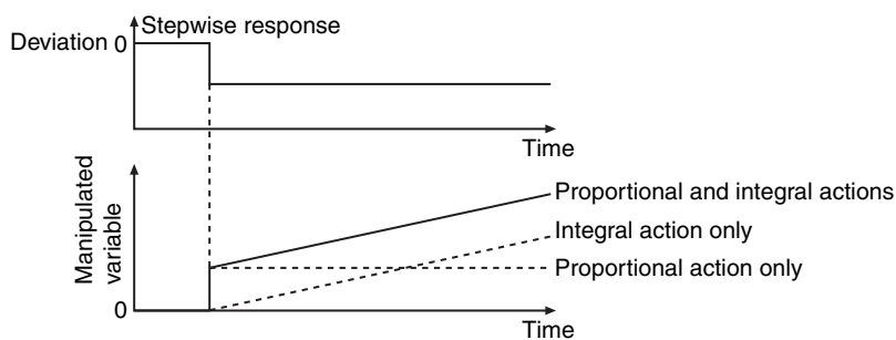
Manipulated Variable for Integral and Proportional Actions Together
