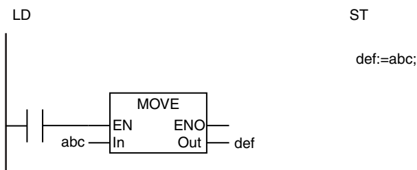
Moving the Entire Structure
