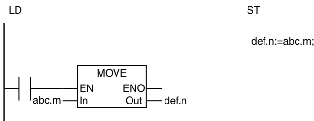
Moving the Entire Structure
