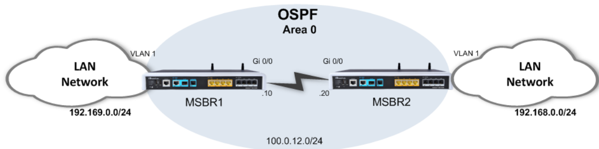
Figure 12-2: OSPF Routing
