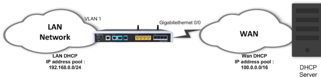
Figure 5-1: DHCP
