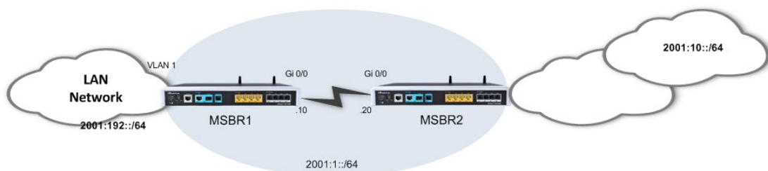
Figure 21-1: Static Routing
