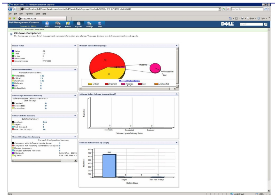
Figure 7. The Altiris Server Management Suite showing the state of Windows compliance before patching the servers.
