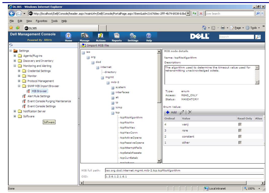
Figure 9. Browsing an MIB in the Dell Management Console.
