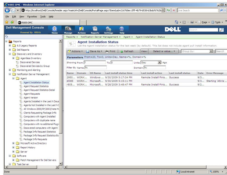
Figure 3. Viewing the installation status.
