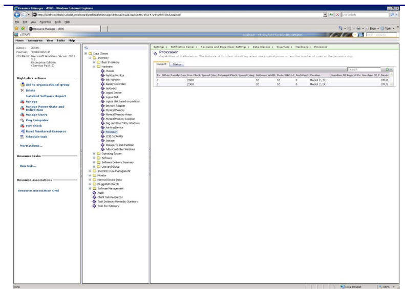
Figure 5. Reviewing inventory information in the Altiris Server management Suite.
