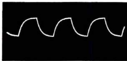
Output from an amplifier having good high-frequency response, indicated by the steep sides of the waveform and good low frequency response indicated by the flat tops of the waveform
