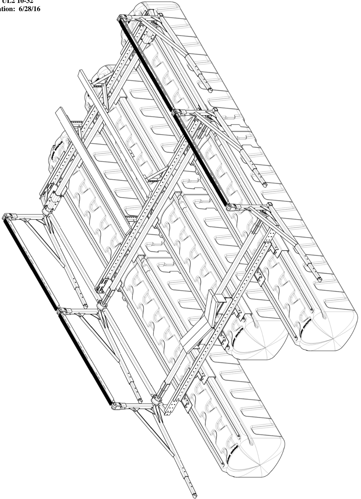
Figure VII-16,000 UL2-Model-16' Slip-3T-6 Arm
