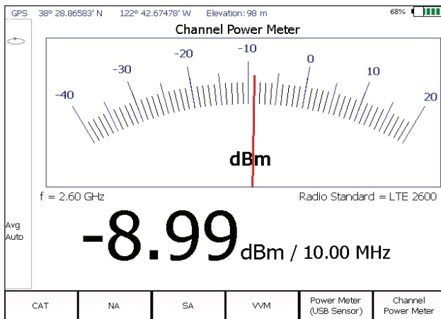
Channel power measurements are easily displayed on a large analog display, viewed in "Outdoor Sun" display mode
