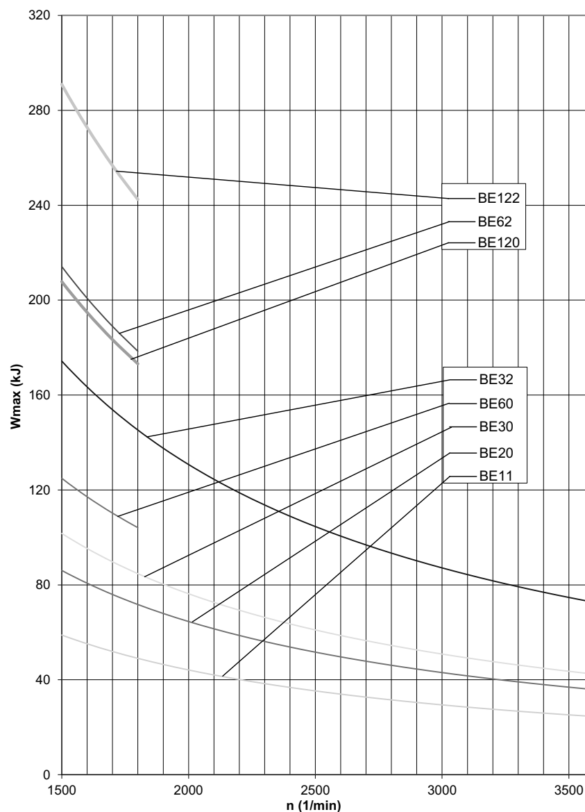
Diagram: Maximum braking work for emergency switching off for travel drives.
