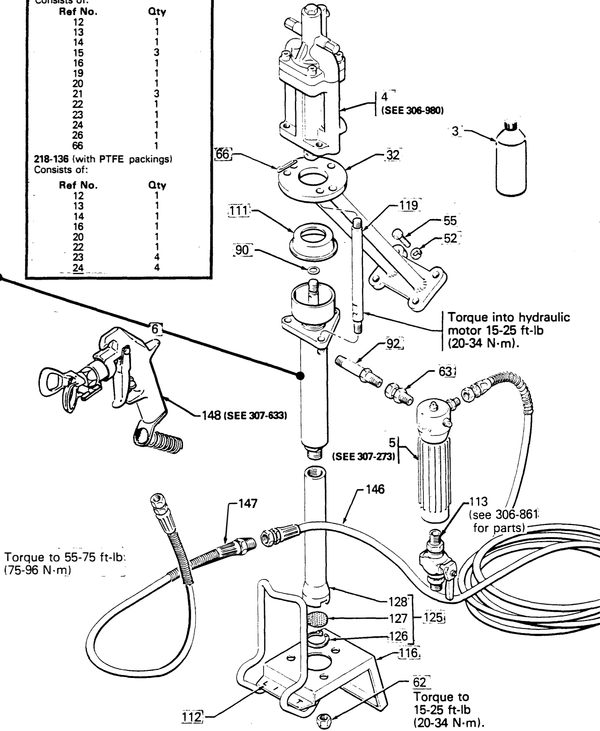
Ref No. 129 5 gal. (19 liter) Suction Tube Assy.
