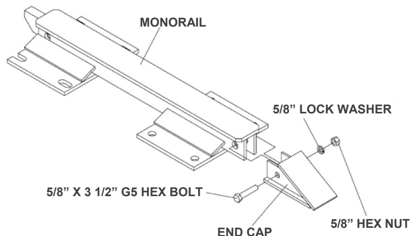
Figure 21 Monorail End Cap Attachment
