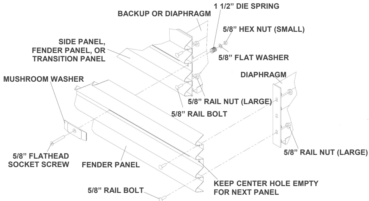
Figure 19 Fender Panel Assembly
