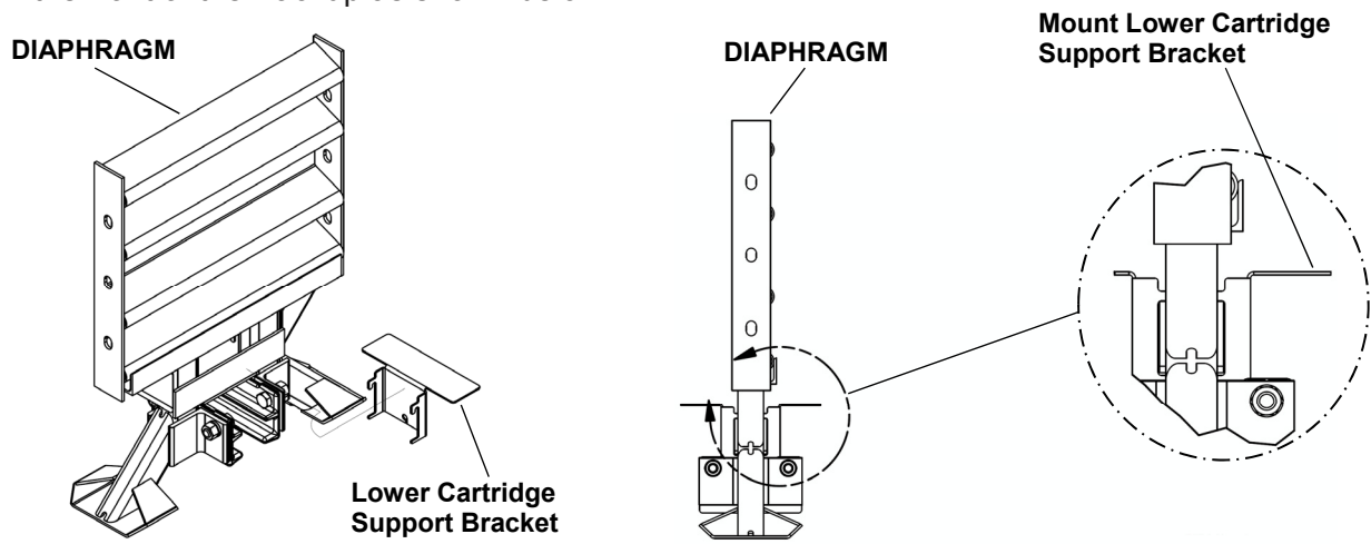
Figure 22 Lower Cartridge Support Bracket Assembly
