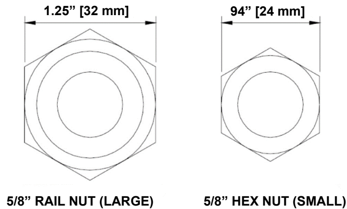
Figure 18 Rail Nuts are Oversize
