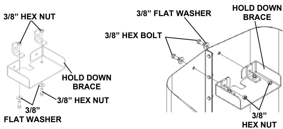
Figure 25 Hold Down Brace Assembly
