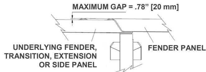
Figure 29 Fender Panel Gap
