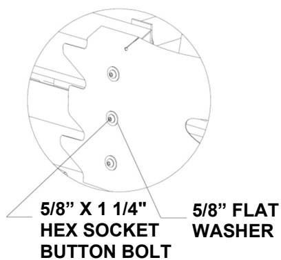
Detail 24a Fastener Assembly
