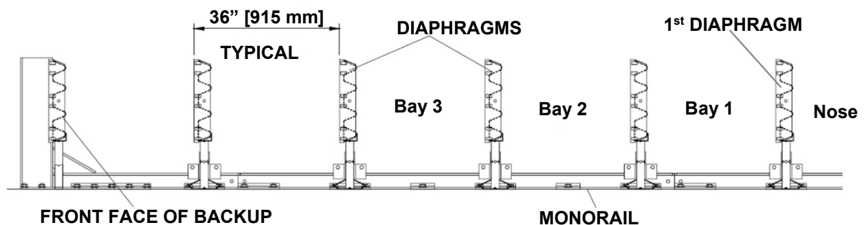
Figure 17 Diaphragm Spacing
