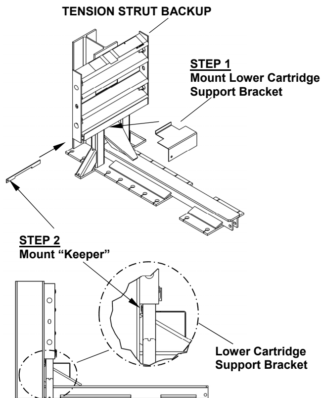
Figure 23 Lower Cartridge Support Bracket Assembly (Tension Strut Backup)
