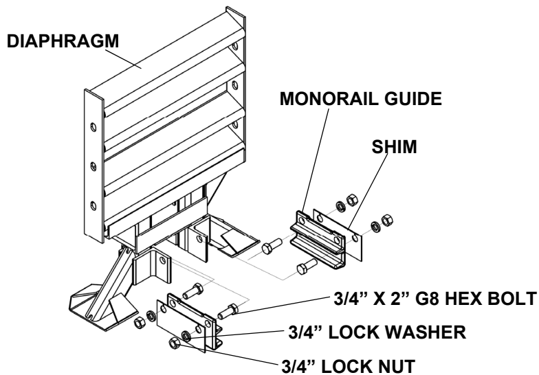
Figure 15 Monorail Guide Attachment
