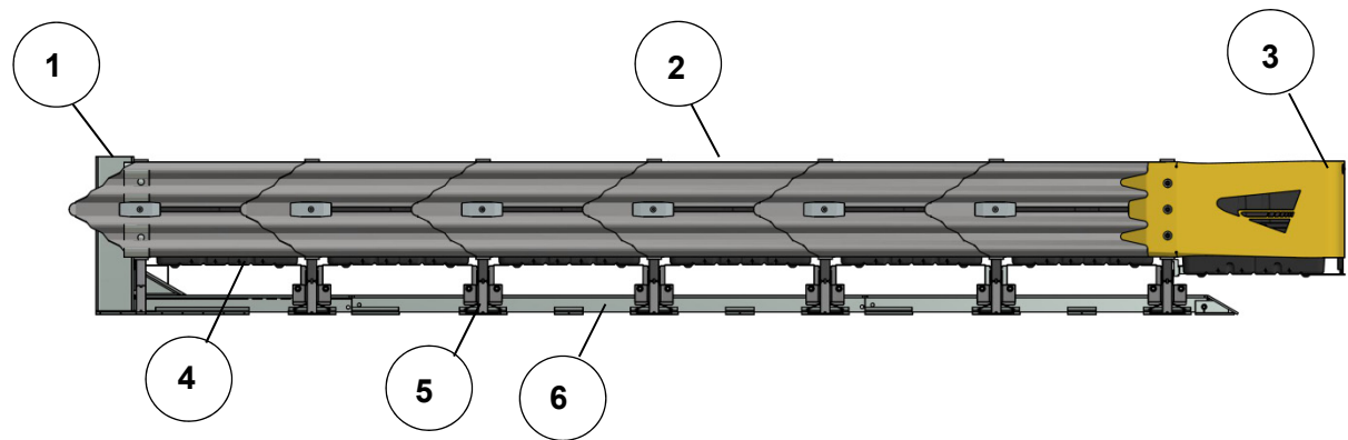
Figure 6 Elevation View
