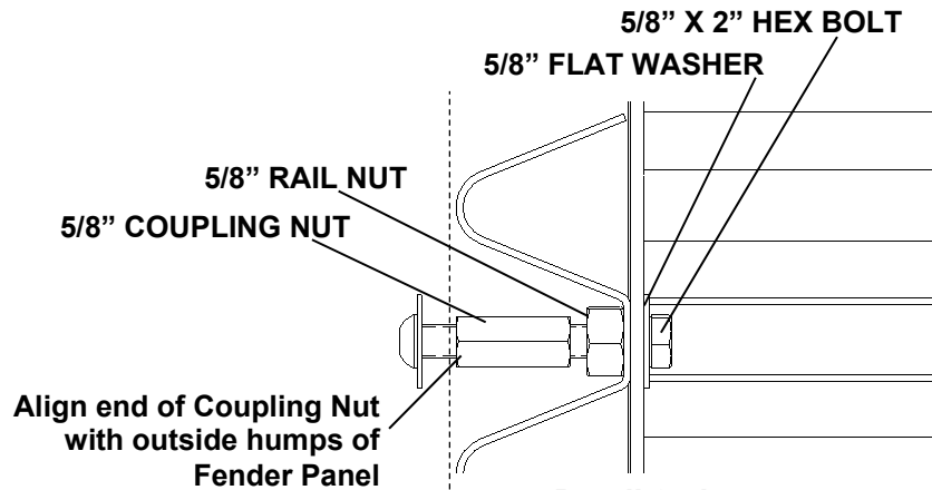
Detail 24d Inside View: Nose Cover Cut Away
