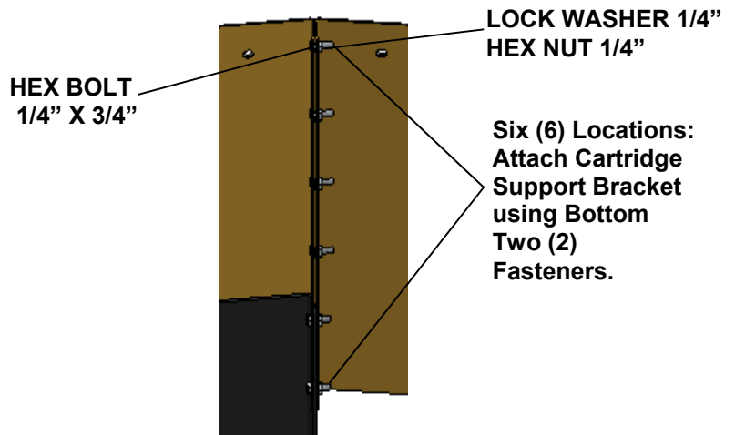
Detail 24f
