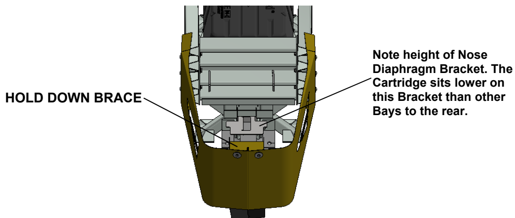
Detail 24g
