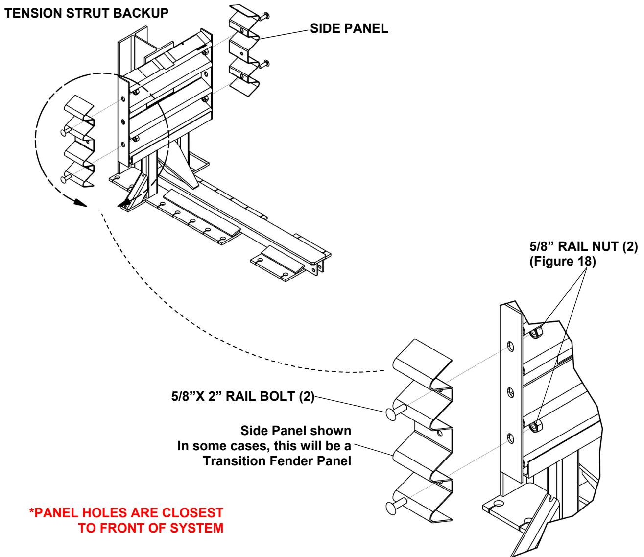
Figure 11 Side Panel/Transition Panel Attachment
