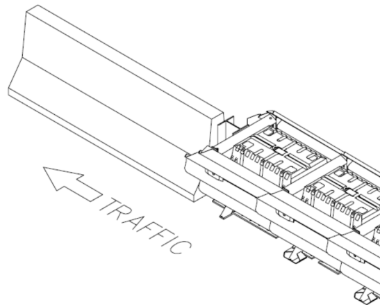
Figure 1 No Transition
