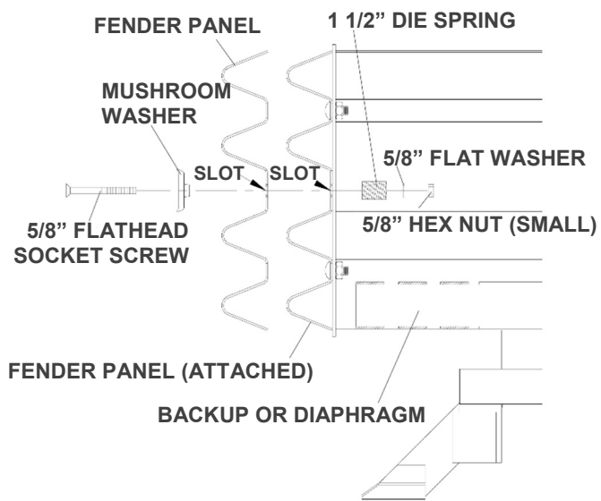
Detail 19a Mushroom Washer Attachment
