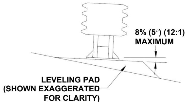
Figure 2 Cross-Slope
