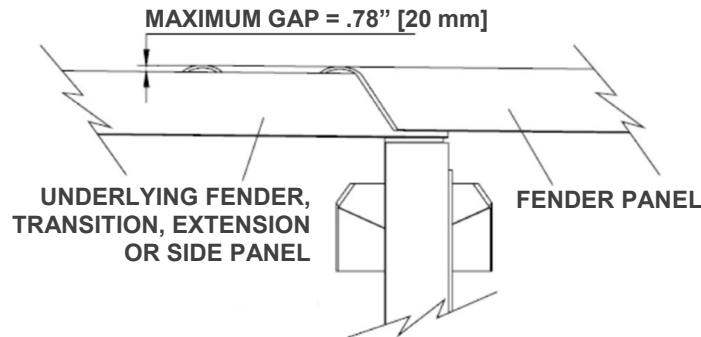
Figure 27 Fender Panel Gap
