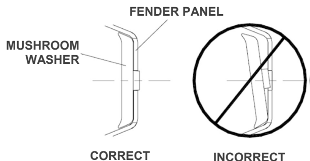
Detail 19b Mushroom Washer Orientation
