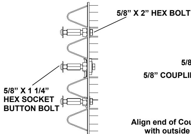
Detail 24c End View: Nose Cover Removed
