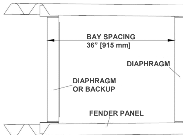
Figure 20 Proper Diaphragm Spacing
