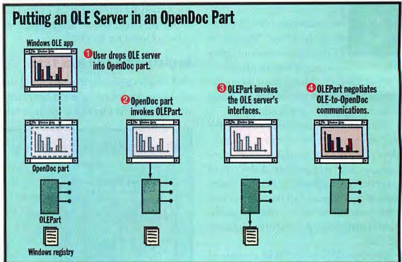
OLEPart lets an OpenDoc part embed an OLE server.
