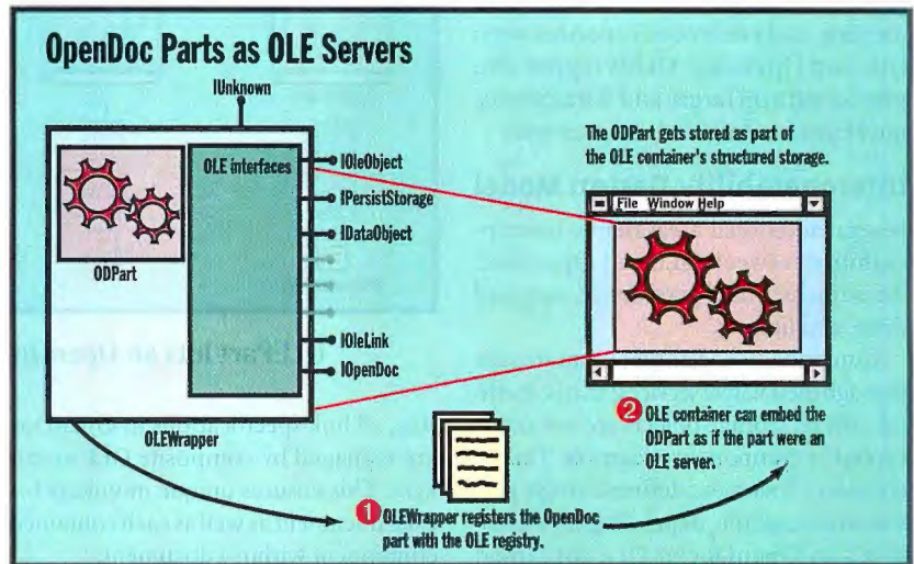
OLEWrapper lets an OLE container embed an OpenDoc part.
