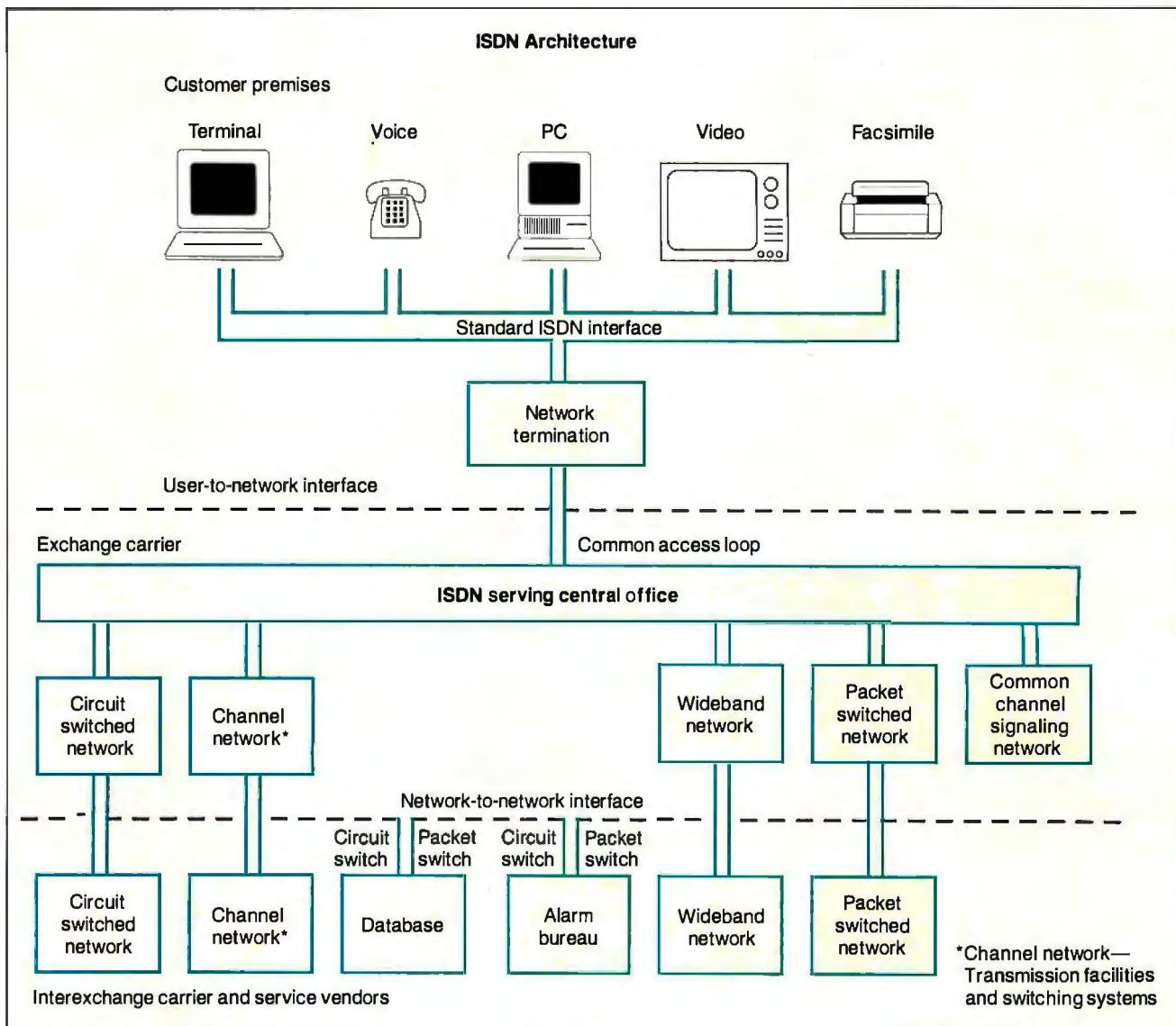
Figure 1: ISDN is an evolving international standard for voice and data communications. Its major features include integrated access of multiple services over a single access line, network transparency via standard customer-to-network and network-to-network interfaces, and end-to-end digital connectivity.
