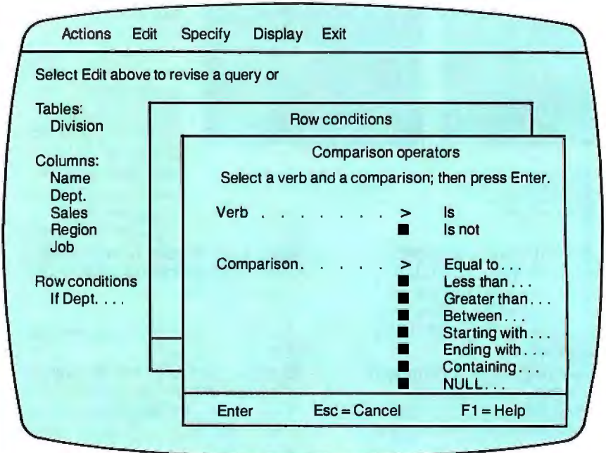
Figure 2: The Extended Edition's Query Manager uses a Prompted Query interface that lets you build valid SQL queries. The left side of the screen shows the query terms already selected, while menus on the right list the possibilities for subsequent terms. Here, the condition "IfDept" could take the verbs "is" or "is not" and the comparison operators "equal to," "less than," and so on.
