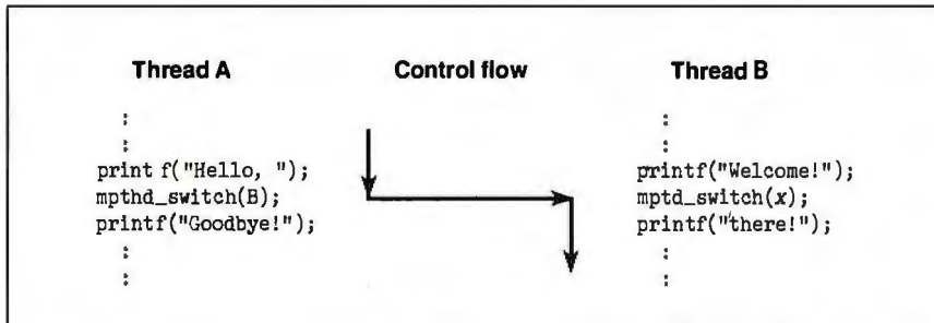
Figure 1: Context switching as performed by mpthd_switch() . The output from this context switch would be "Hello, there!"; "Hello," comes from thread A, which switches to thread B for "there!".
