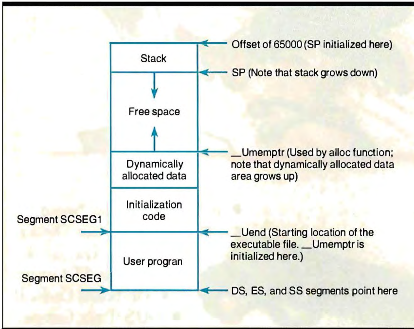
Figure 1: BYTE Small-C's memory map.
