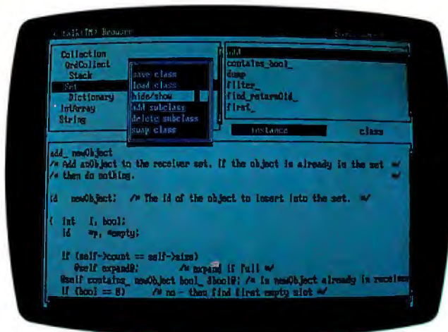
C_talk features a Smalltalk-like browser.
