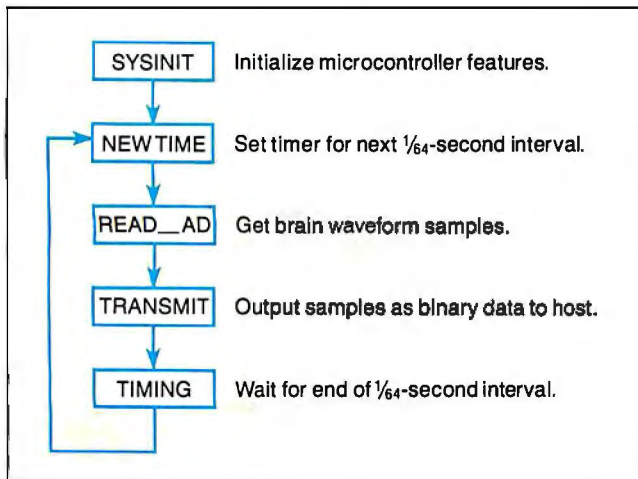
Figure 2: A flowchart for HAL's firmware program, BIO31.
