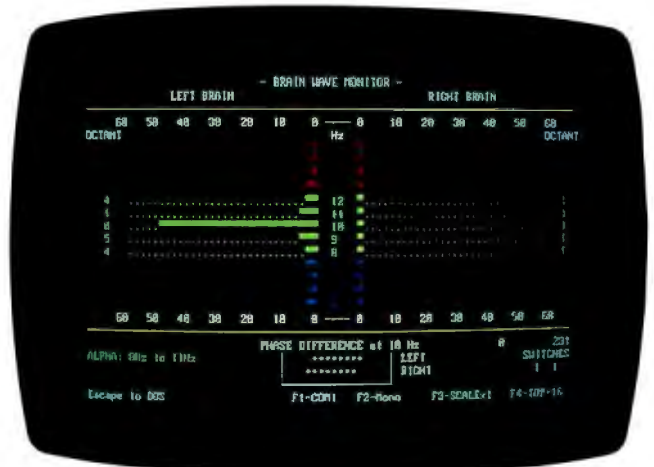
Photo 3: While testing HAL, I injected a 10-Hz sine wave through the headset electronics. The resulting output, shown here, indicates that the system works properly.
