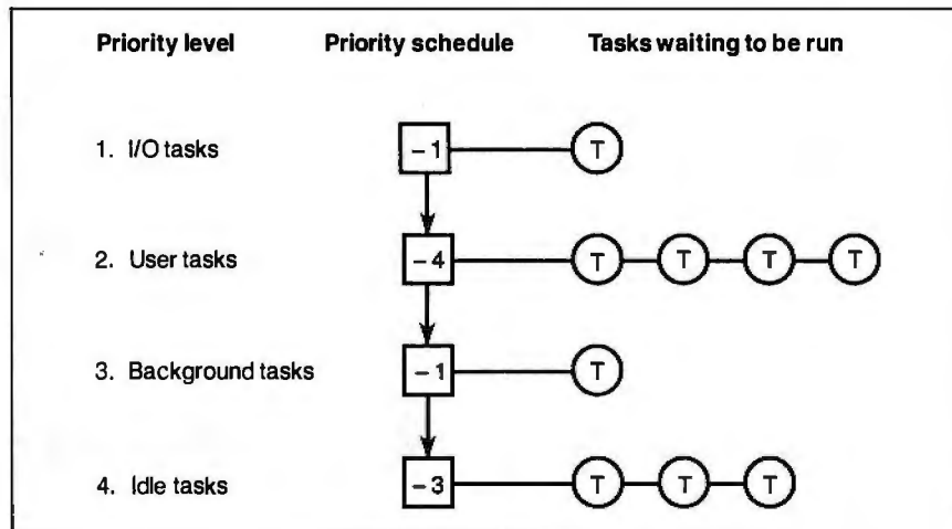
Figure 5: A mailbox scheduler example. To find a new task to run, a processor simply searches down the schedule list until it finds a task.
