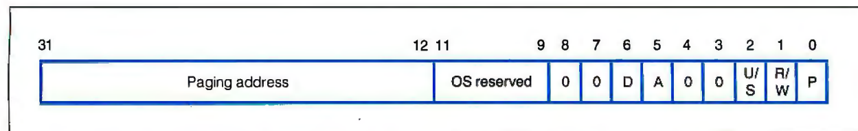
Figure A: Page-directory entry and page-table entry layout. PDEs and PTEs are almost identical, but a PDE points to a page table, while a PTE points to a page.
