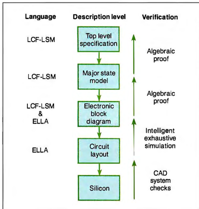
Figure 3: VIPER's hardware validation process uses a hierarchy of description levels.
