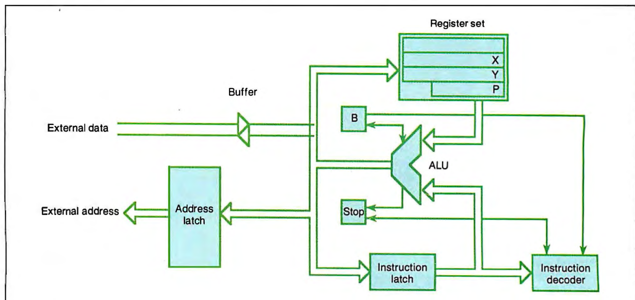
Figure 1: Proving the mathematical correctness of the VIPER-1 microprocessor required a simple architecture, as shown here.
