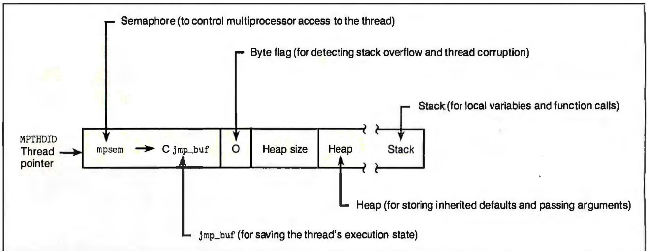
Figure 2: Internal representation of the thread data type.
