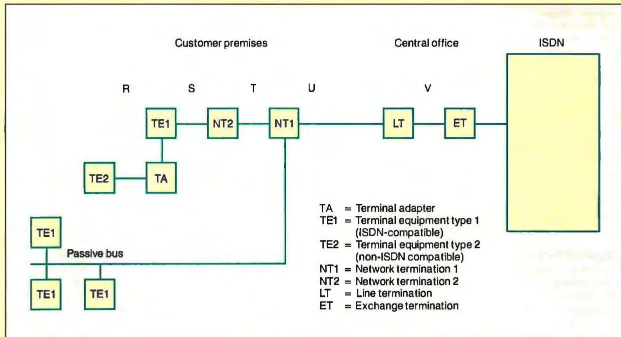
Figure A: The CCITT, a communications governing body of the United Nations, has designated five ISDN reference points: R, S, T, U, and V. These are places in the network where one or more interfaces for specific functions will occur.
