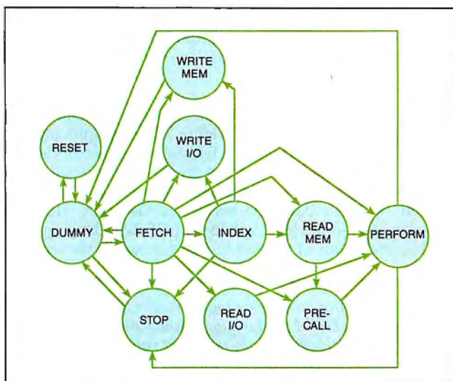
Figure 2: Eleven major states represent the mathematical model of the VIPER microprocessor.
