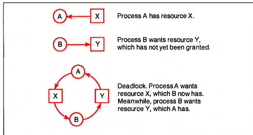
Figure A: Deadlock will occur if and only if a cycle exists in the resource-allocation graph.
