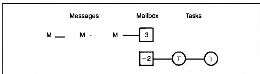
Figure 4: Mailbox "message bank." The upper diagram is of a mailbox with messages waiting for tasks (positive count); the lower diagram is of a mailbox with tasks waiting for messages (negative count).
