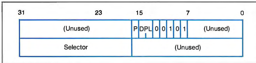
Figure 1: The task-gate descriptor. A procedure may gain access to a task through a task gate rather than the task-gate segment. Once it passes the privilege-level check at the task gate, no further protection checking takes place.
