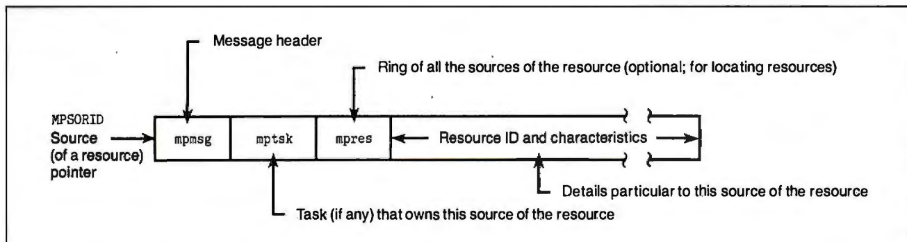
Figure 6: Internal representation of a source (of a resource) data type.
