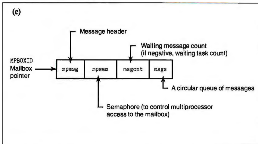
Figure 3: Internal representations of the (a) tasks, (b) messages, and (c) mailboxes data types.
