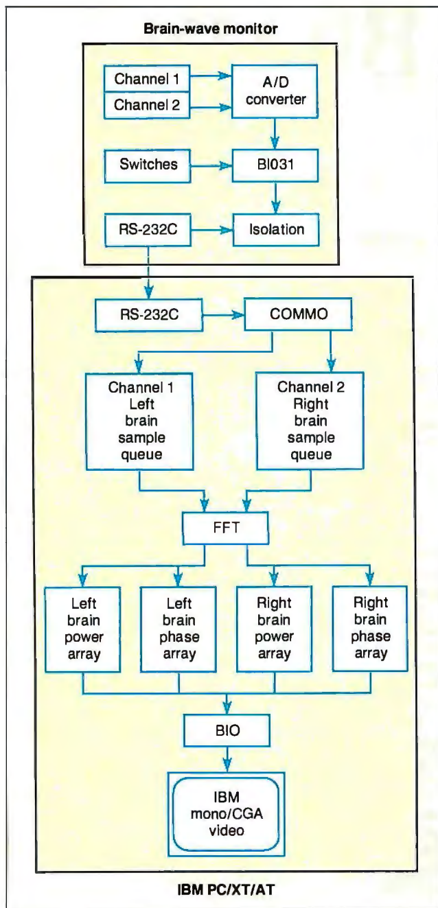
Figure 1: A block diagram of the complete HAL system, showing major components of the brain-wave monitor and the host machine.
