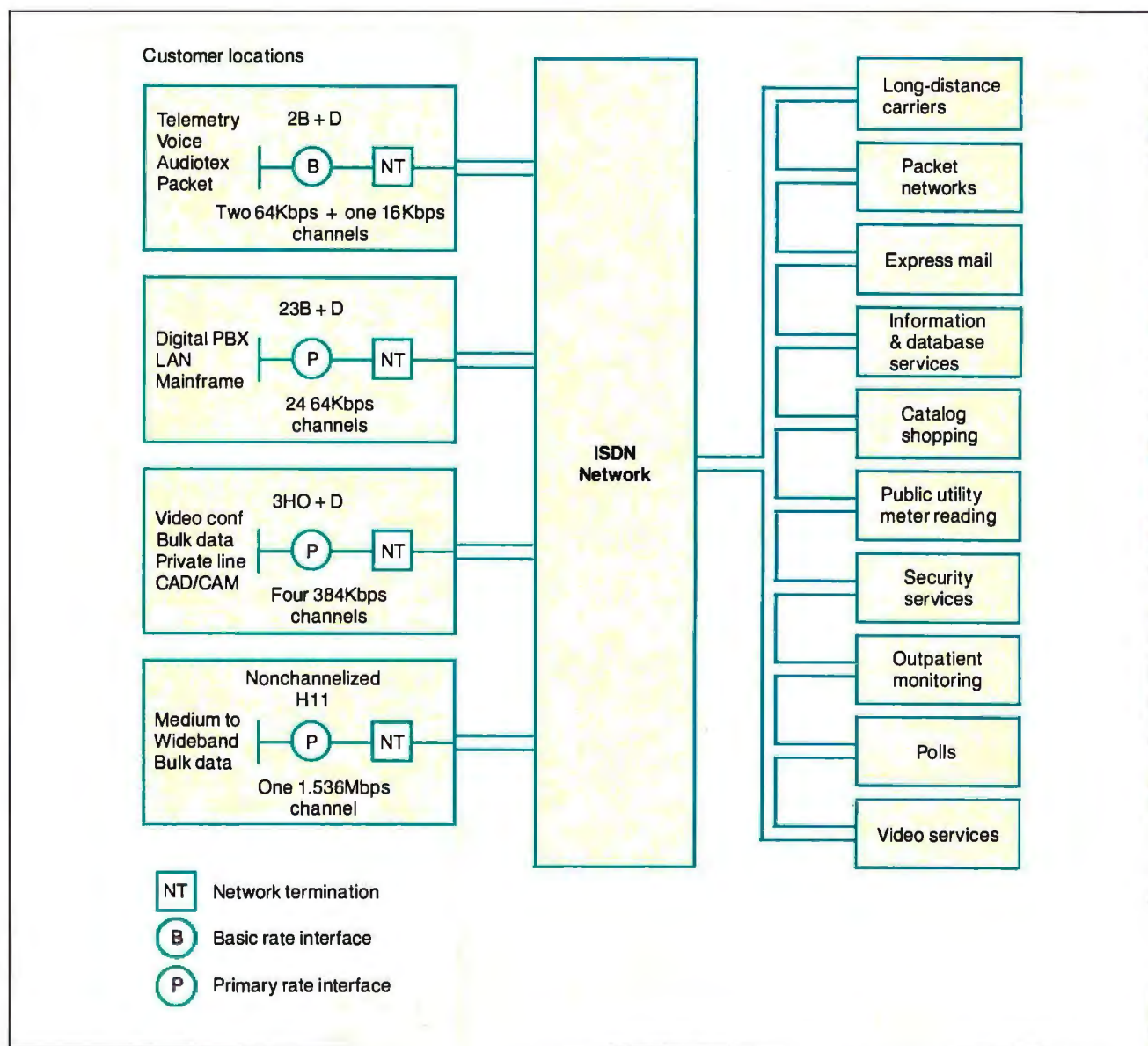
Figure 2: Many services will be available over ISDN's basic and primary rate interfaces when the technology is fully employed. Some of the potential applications are shown here.
