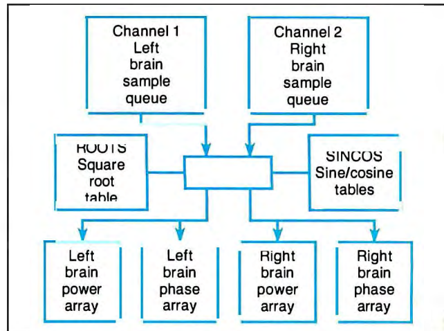
Figure 5: Main components of the FFT.
