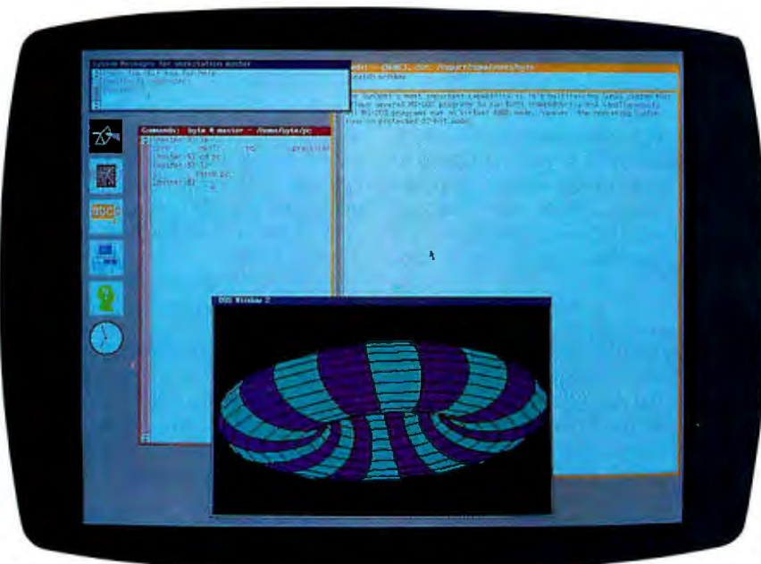
Photo 1: On the SunView Desktop, icons represent active processes, not files.
