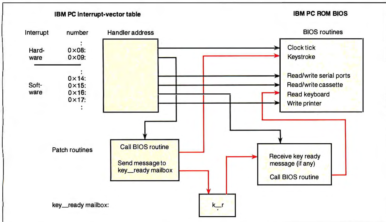
Figure 7: Intercepting interrupts (advanced optimizations). To prevent tasks from wasting processor time waiting for keystrokes, you can intercept the IBM PC’s BIOS interrupt routines to check and signal when a keystroke has occurred. Since you can call Mailbox’s send and receive primitives within interrupts, many such schedule optimizations are possible without rewriting the scheduler.
