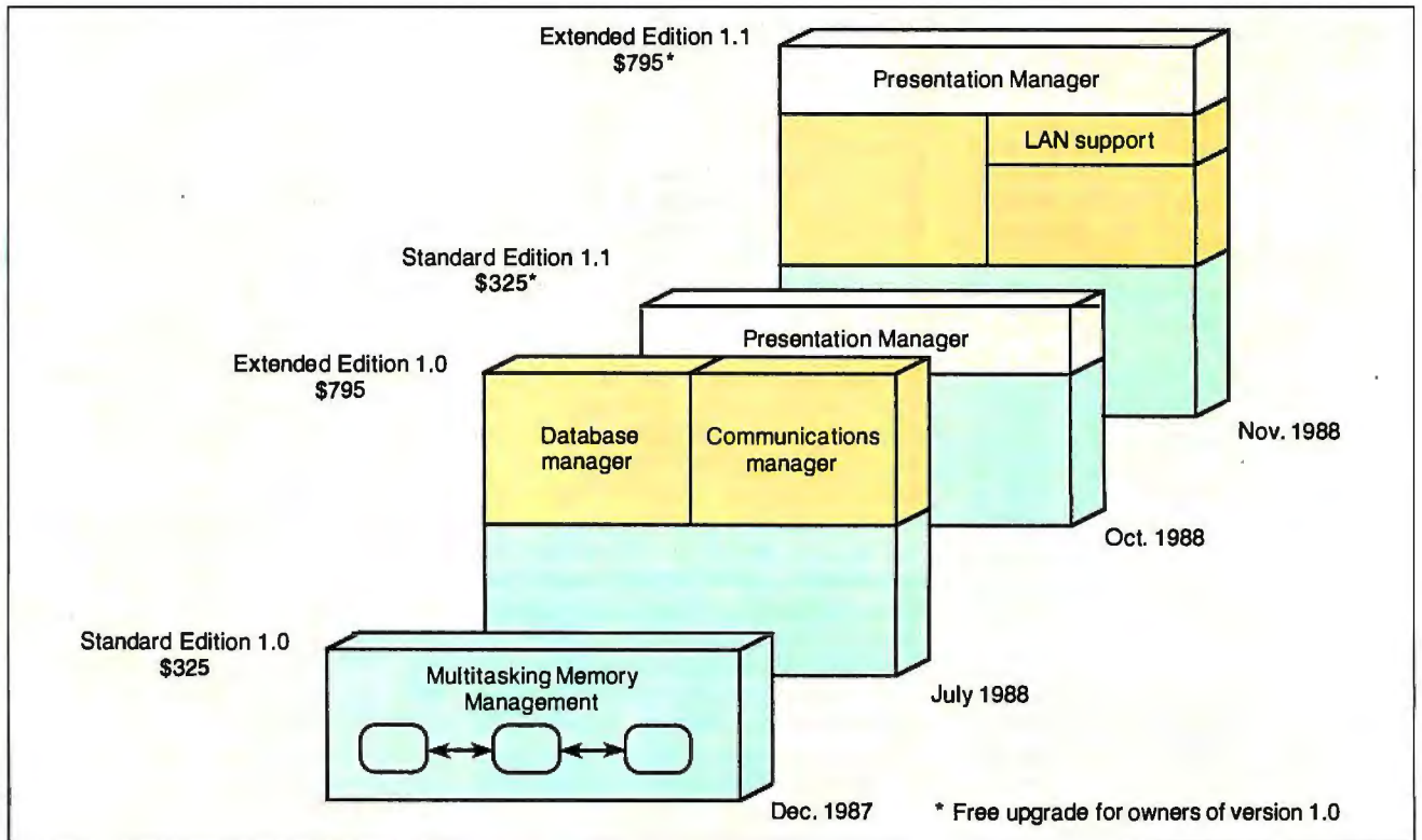
Figure 1: The Extended Edition of OS/2 adds database and communications managers to the base operating system of the Standard Edition. Later this year, both editions will be upgraded to include the Presentation Manager, a Windows-like graphic user interface.
