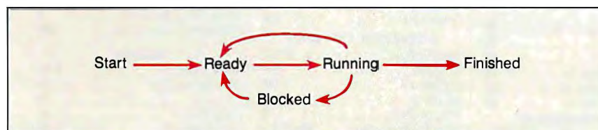
Figure 1: The various state changes that can occur as a task proceeds from start to finish.
