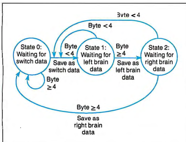
Figure 3: The host computer's receiver routine executes a finite-state machine, shown here graphically. Each circular node of the graph represents a state, and transitions from state to state occur when the system receives a byte.
