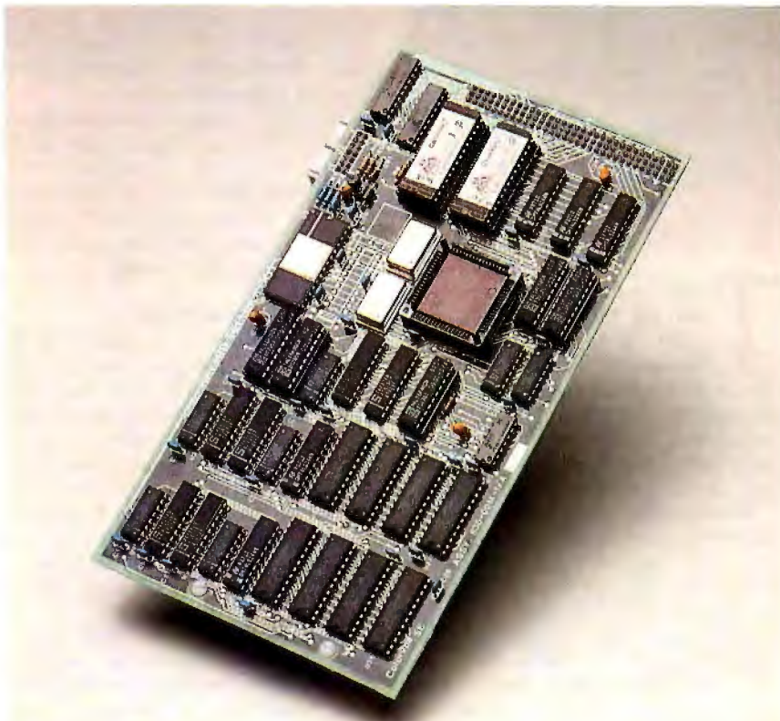
Photo 1: The ColorVue SE add-on board, with 2 megabytes of video RAM.
