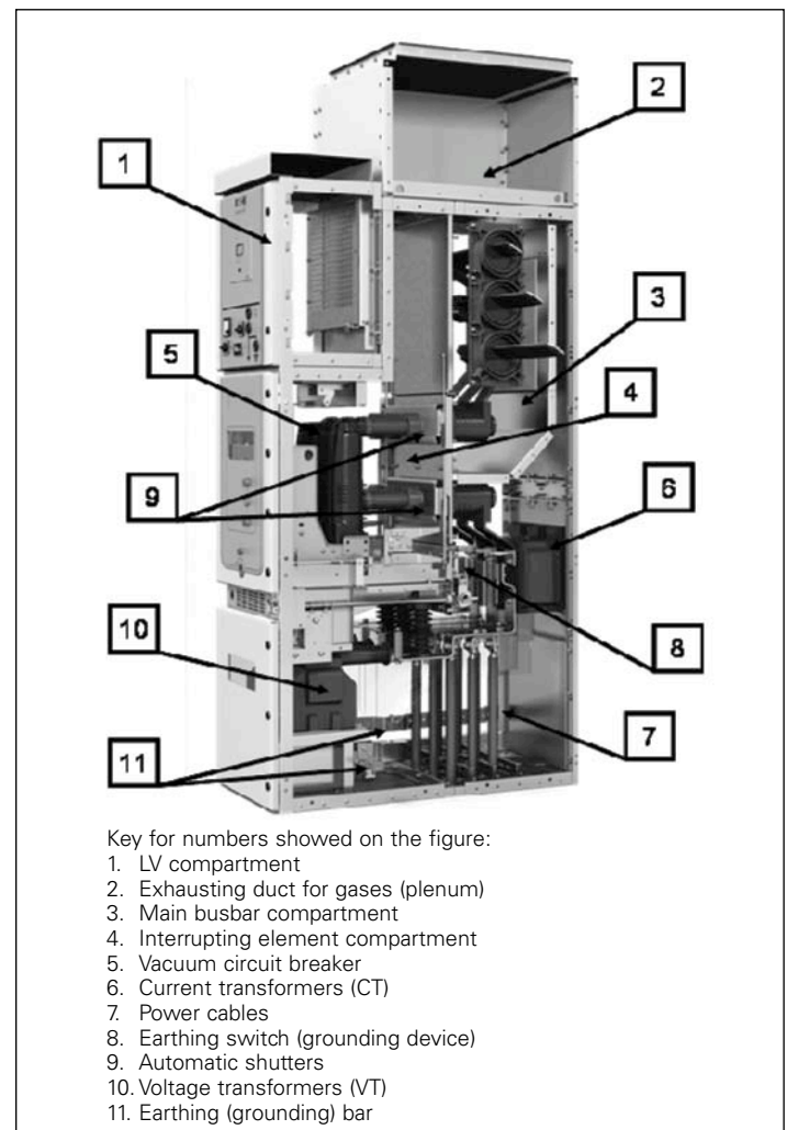
Figure 16. An Example of Modern MV Metal-Enclosed Indoor Air-Insulated Withdrawable Switchgear Unit Design Philosophy Adopted by the Brazilian Petrochemical Sector
