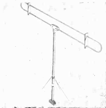
Camco "Featherlite" folded dipole, Model F22 for 88 to 108 mc FM band, with or without twin lead. Model T32 covers 44 to 216 mc for tele.
