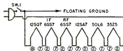
Fig. 3. New Arvin wiring prevents 6S57 burnouts.
