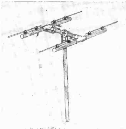
JFD standard dipole with reflector.
