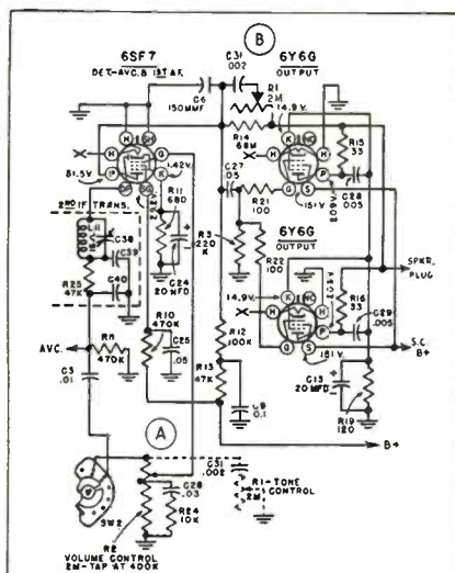
Fig. 2. Westinghouse tonal range is increased by moving control from position A to point B.
