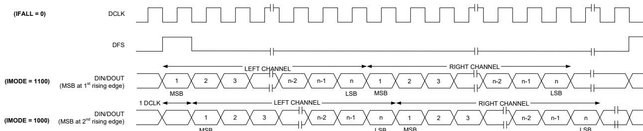
Figure 27. DSP Digital Audio Format
