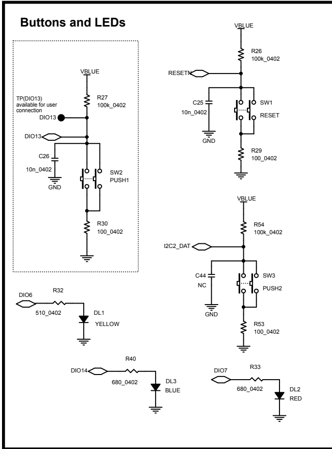
Figure 59. STEVAL-IBD008V1M circuit schematic (2 of 3)
