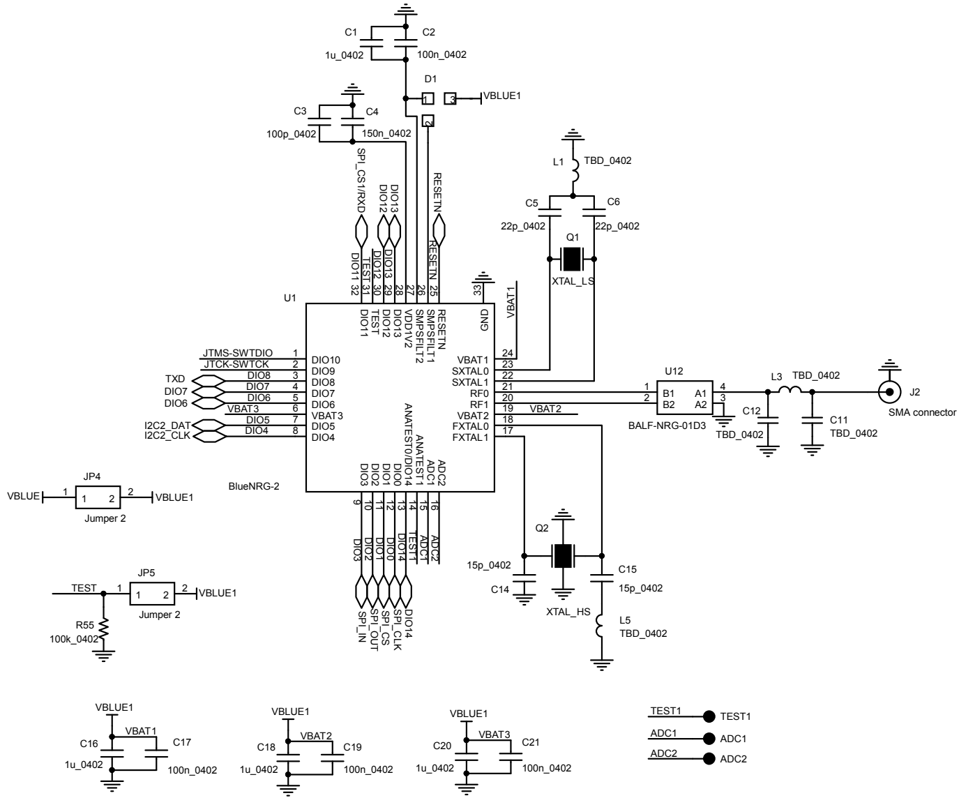
Figure 37. STEVAL-IDB008V1 circuit schematic - BlueNRG-2
