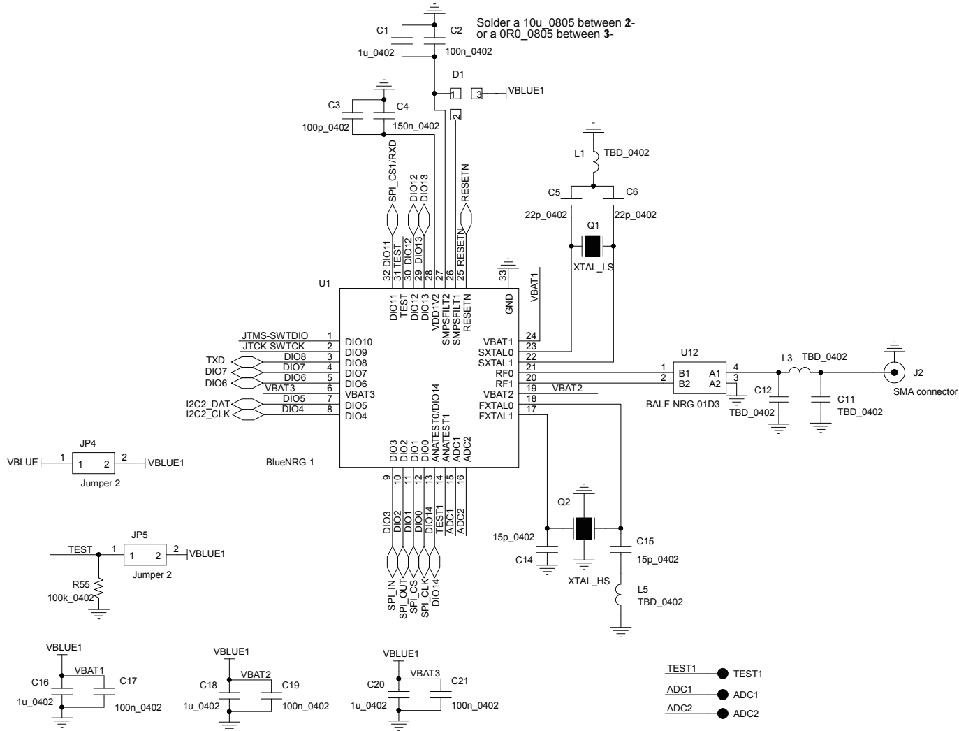
Figure 26. STEVAL-IDB007V1 BlueNRG-1
