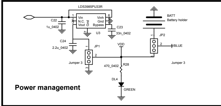
Figure 59. STEVAL-IBD008V1M circuit schematic (2 of 3)
