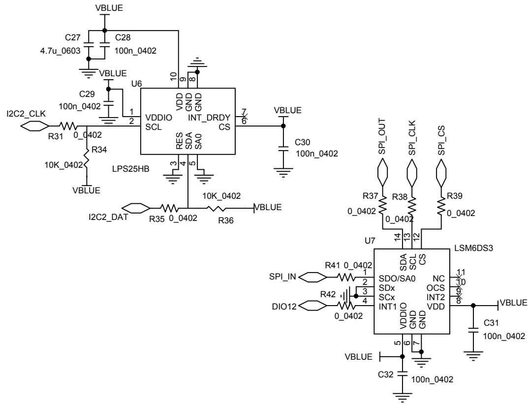
Figure 51. STEVAL-IDB008V2 - SENSORS
