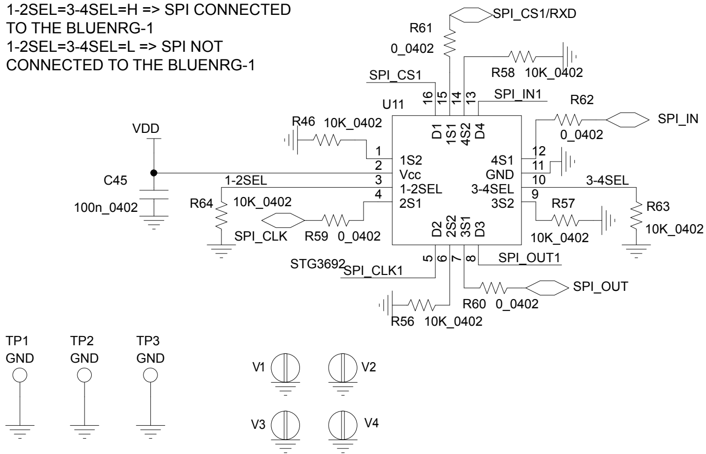
Figure 31. STEVAL-IDB007V1 switch
