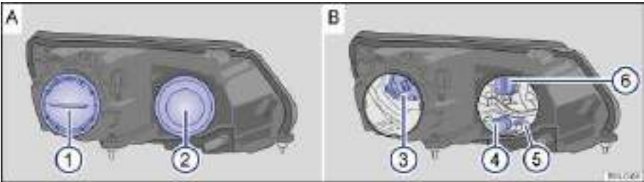
Fig. 200 In the engine compartment: Cover 1 on the left headlight for the low beam bulb holder 3 and cover 2 for the parking light bulb holder 4, turn signal bulb holder 5 and high beam or daytime running light bulb 6.
