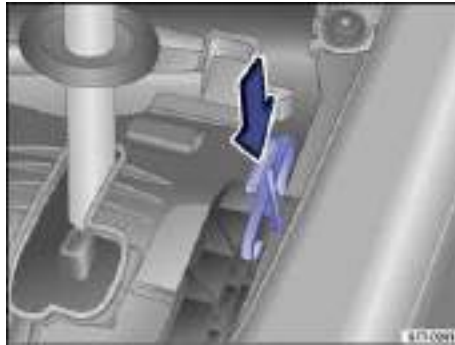
Fig. 183 Releasing the selector lever lock.
