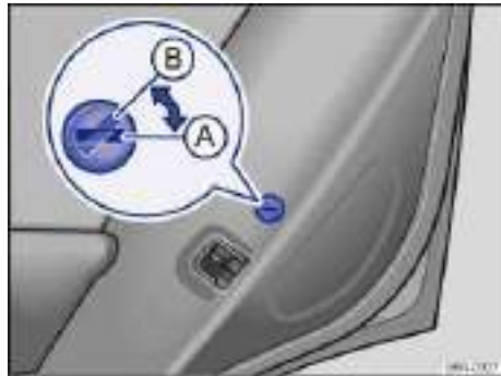
Fig. 30 In the right rear door: Child safety lock A deactivated, B activated.
