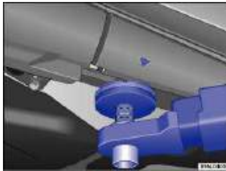
Fig. 176 Rear lift point for workshop hoist or floor jack.
