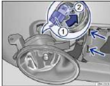
Fig. 203 Replacing light bulb in headlight.
