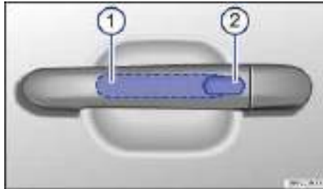
Fig. 28 Keyless Access locking and starting system: Sensor 1 for unlocking on the inside of the front door handles. Sensor for locking 2 on the outside of the door handles.
