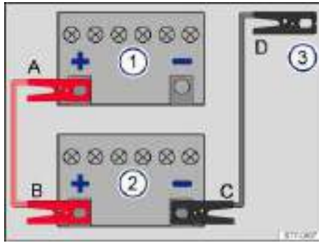
Fig. 210 Diagram for attaching the jumper cables: Dead battery 1 and booster battery 2.
