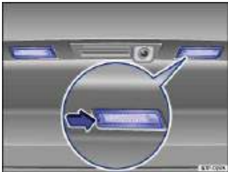
Fig. 208 In the rear hatch: Clamped license plate lamp.
