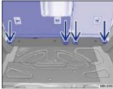
Fig. 99 Rear attachment of the rear seat.
