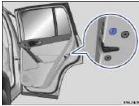
Fig. 179 On the front side of the right rear door: Emergency lock, covered by a rubber seal.
