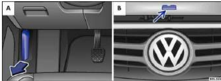
Fig. 162 A: Inside engine hood release in the footwell on the driver side. B: Outside engine hood release in the radiator grille.
