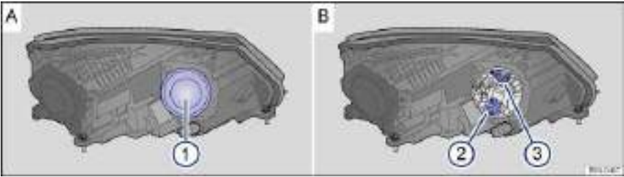
Fig. 201 In the engine compartment: cCover 1 on the left headlight for the turn signal bulb holder 2 and the cornering light bulb holder 3.
