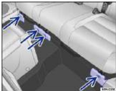
Fig. 98 Front attachment of the rear seat.
