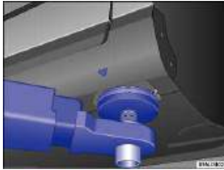
Fig. 175 Front lift point for workshop hoist or floor jack.
