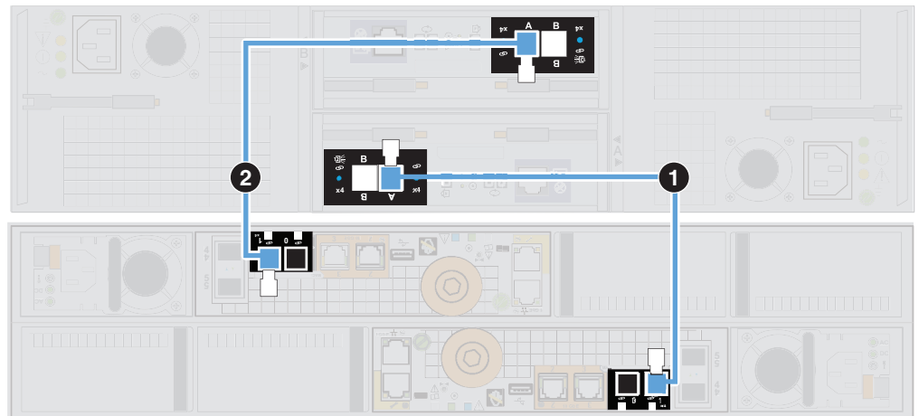
DPE to 15-drive DAE SAS cabling
