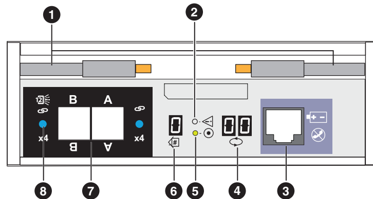
Figure 21 2U, 25-drive DAE LCC ports, LEDs, and connectors
