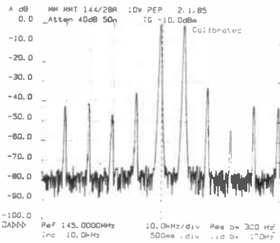
Fig 4 10W two-tone intermod
