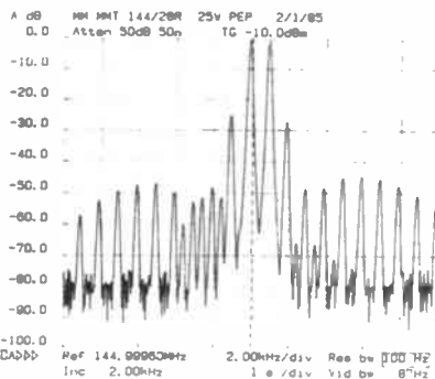
Fig 5 25W two-tone intermod
