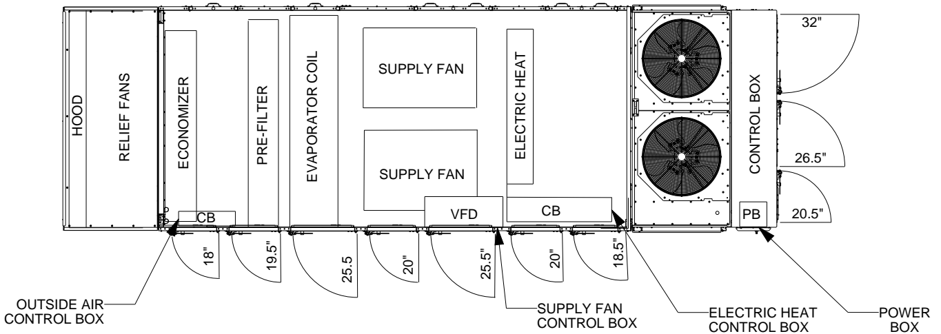
Figure 45. Minimum access clearances – 20 to 30 ton
