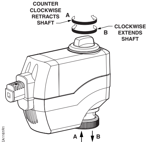
Figure 7. Manual Override.
