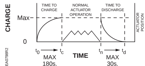
Figure 1. SSC81.5U Electronic Spring Return Mechanism.
